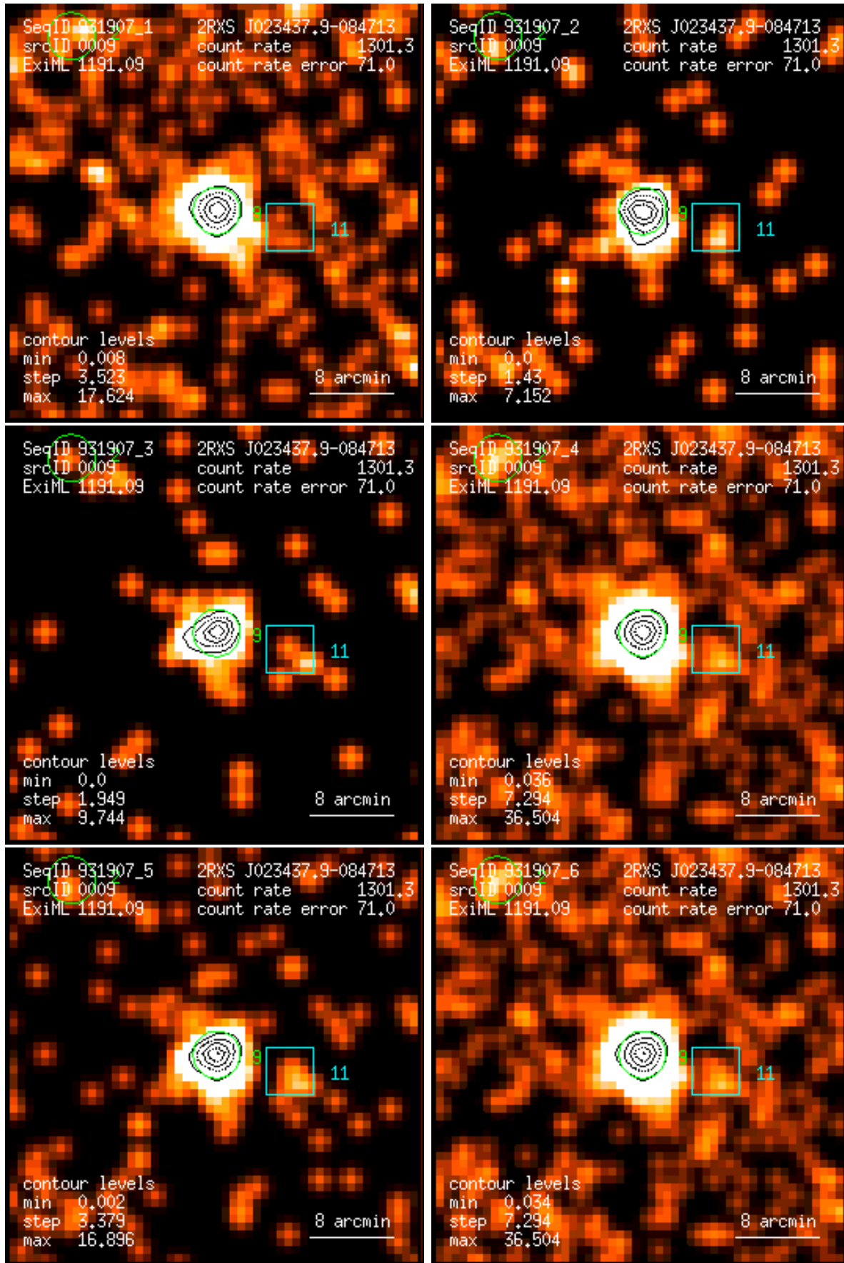
Figure 9: RASS 931907: detection 0009: band rate images, Gaussian filter: (1) PSPC channels 11 – 41, (2) 52 – 90, (3) 91 – 201, (4) 11 – 235, (5) 52 – 201, (6) 11 – 201. Broad band rates in counts/ks. Band rate contour levels in counts/ks/arcmin 2 .
