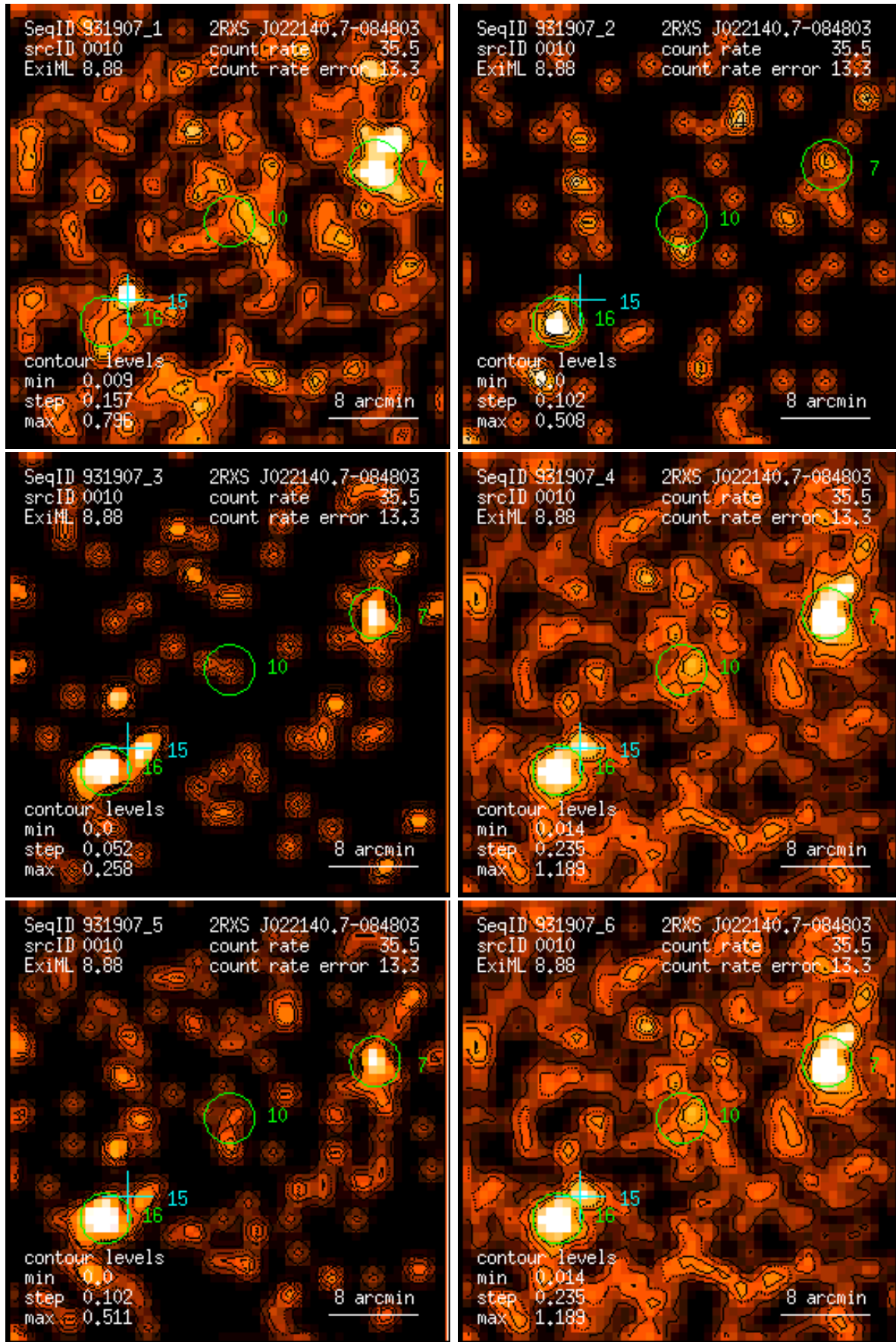
Figure 10: RASS 931907: detection 0010: band rate images, Gaussian filter: (1) PSPC channels 11 – 41, (2) 52 – 90, (3) 91 – 201, (4) 11 – 235, (5) 52 – 201, (6) 11 – 201. Broad band rates in counts/ks. Band rate contour levels in counts/ks/arcmin 2 .
