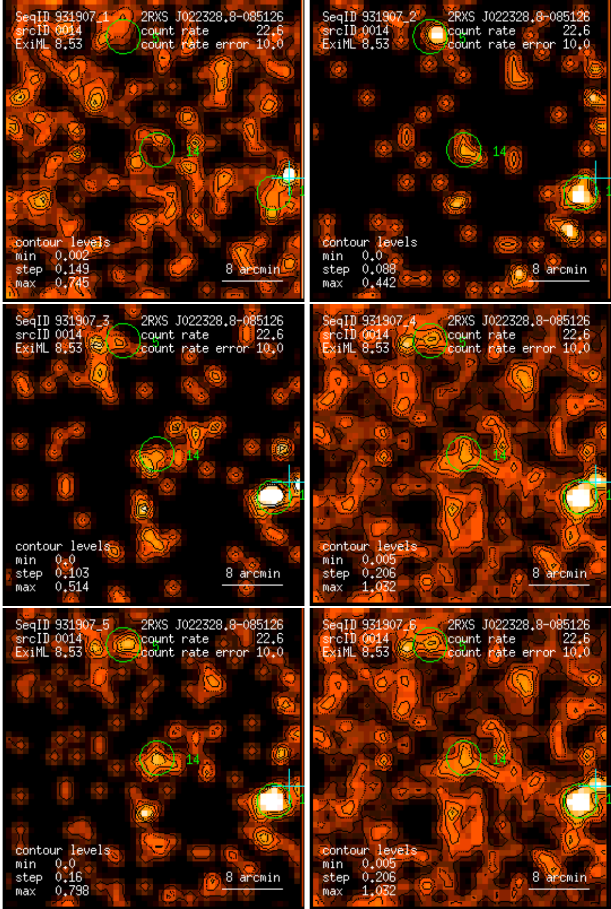
Figure 14: RASS 931907: detection 0014: band rate images, Gaussian filter: (1) PSPC channels 11 – 41, (2) 52 – 90, (3) 91 – 201, (4) 11 – 235, (5) 52 – 201, (6) 11 – 201. Broad band rates in counts/ks. Band rate contour levels in counts/ks/arcmin 2 .
