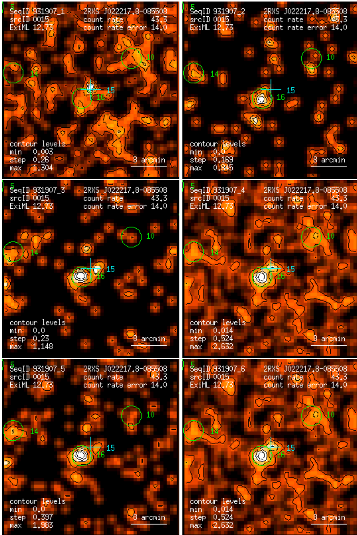
Figure 15: RASS 931907: detection 0015: band rate images, Gaussian filter: (1) PSPC channels 11 – 41, (2) 52 – 90, (3) 91 – 201, (4) 11 – 235, (5) 52 – 201, (6) 11 – 201. Broad band rates in counts/ks. Band rate contour levels in counts/ks/arcmin 2 .
