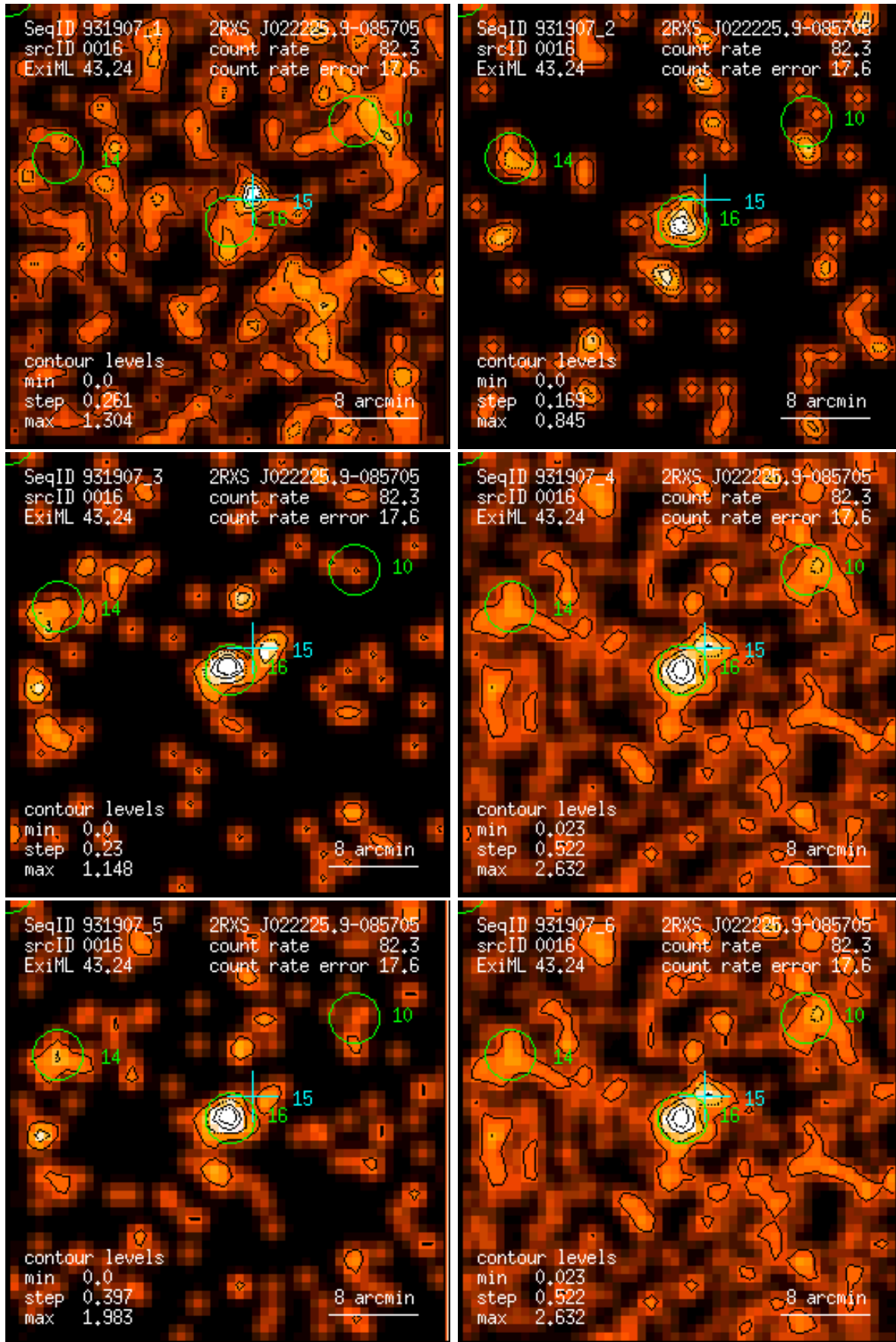
Figure 16: RASS 931907: detection 0016: band rate images, Gaussian filter: (1) PSPC channels 11 – 41, (2) 52 – 90, (3) 91 – 201, (4) 11 – 235, (5) 52 – 201, (6) 11 – 201. Broad band rates in counts/ks. Band rate contour levels in counts/ks/arcmin 2 .
