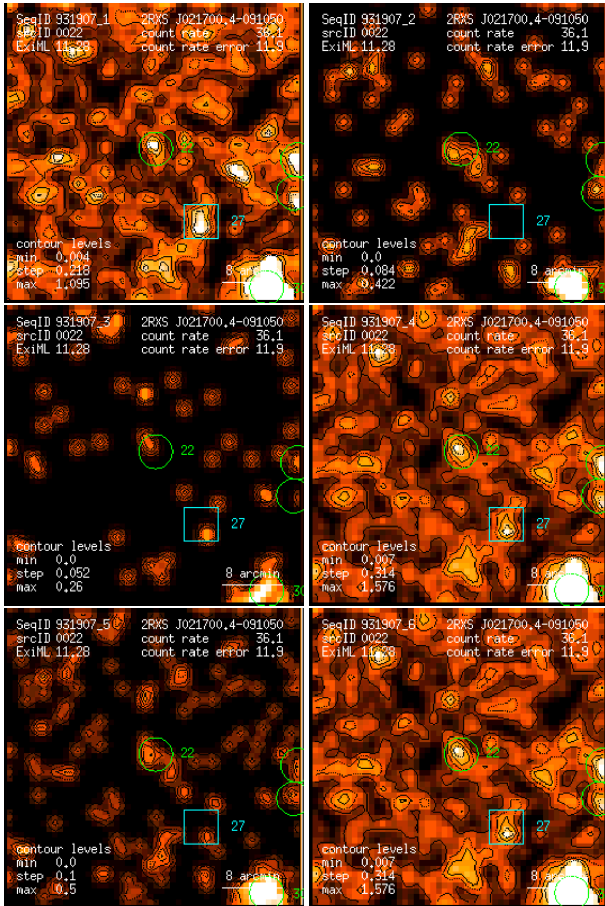
Figure 22: RASS 931907: detection 0022: band rate images, Gaussian filter: (1) PSPC channels 11 – 41, (2) 52 – 90, (3) 91 – 201, (4) 11 – 235, (5) 52 – 201, (6) 11 – 201. Broad band rates in counts/ks. Band rate contour levels in counts/ks/arcmin 2 .
