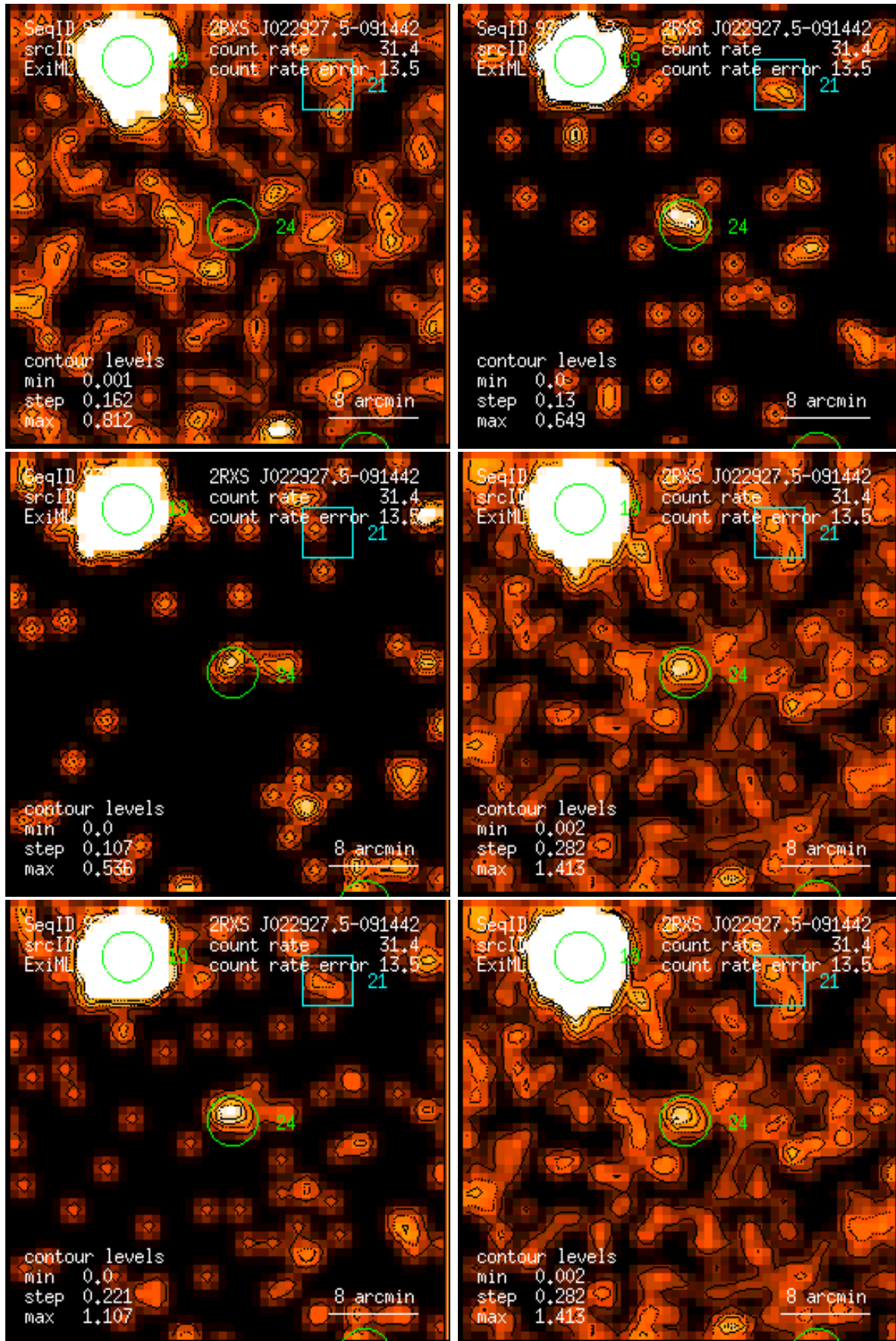
Figure 24: RASS 931907: detection 0024: band rate images, Gaussian filter: (1) PSPC channels 11 – 41, (2) 52 – 90, (3) 91 – 201, (4) 11 – 235, (5) 52 – 201, (6) 11 – 201. Broad band rates in counts/ks. Band rate contour levels in counts/ks/arcmin 2 .
