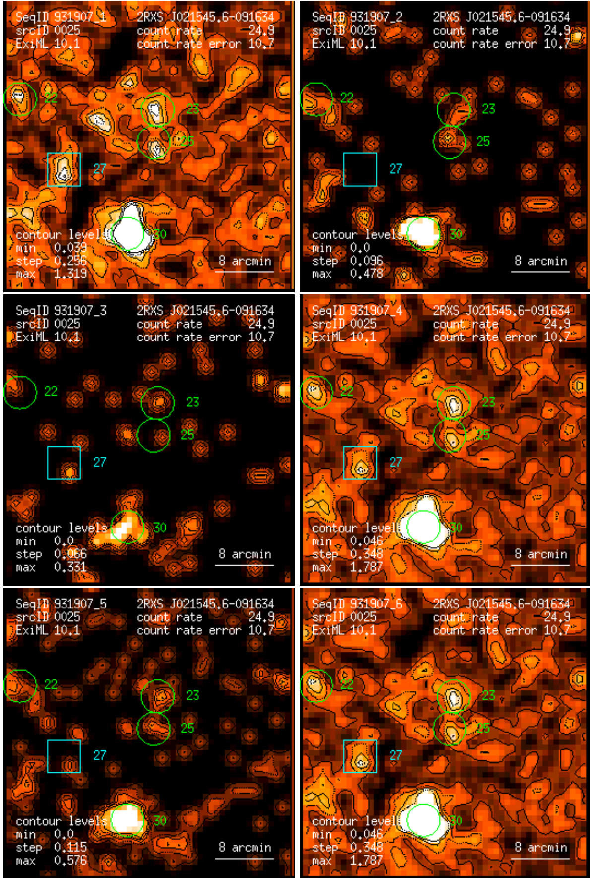
Figure 25: RASS 931907: detection 0025: band rate images, Gaussian filter: (1) PSPC channels 11 – 41, (2) 52 – 90, (3) 91 – 201, (4) 11 – 235, (5) 52 – 201, (6) 11 – 201. Broad band rates in counts/ks. Band rate contour levels in counts/ks/arcmin 2 .
