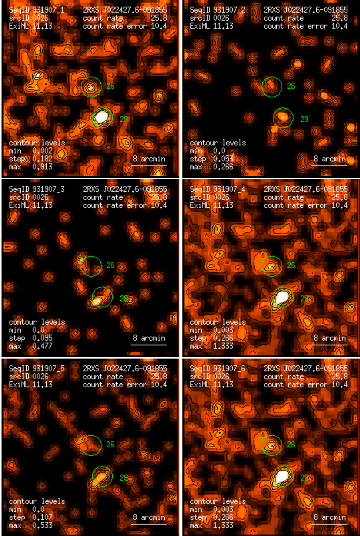
Figure 26: RASS 931907: detection 0026: band rate images, Gaussian filter: (1) PSPC channels 11 – 41, (2) 52 – 90, (3) 91 – 201, (4) 11 – 235, (5) 52 – 201, (6) 11 – 201. Broad band rates in counts/ks. Band rate contour levels in counts/ks/arcmin 2 .
