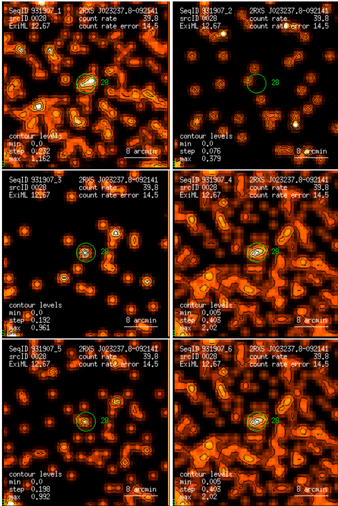
Figure 28: RASS 931907: detection 0028: band rate images, Gaussian filter: (1) PSPC channels 11 – 41, (2) 52 – 90, (3) 91 – 201, (4) 11 – 235, (5) 52 – 201, (6) 11 – 201. Broad band rates in counts/ks. Band rate contour levels in counts/ks/arcmin 2 .
