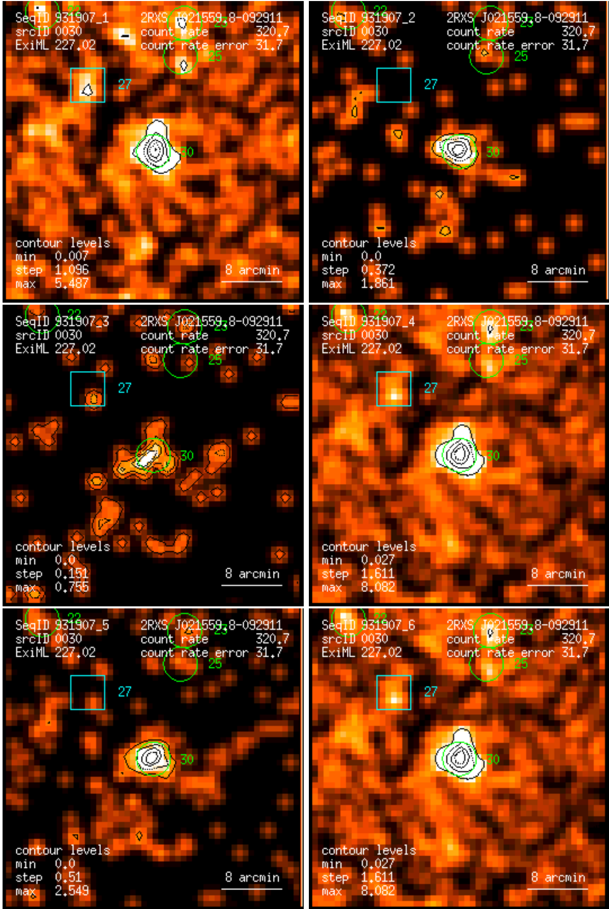
Figure 30: RASS 931907: detection 0030: band rate images, Gaussian filter: (1) PSPC channels 11 – 41, (2) 52 – 90, (3) 91 – 201, (4) 11 – 235, (5) 52 – 201, (6) 11 – 201. Broad band rates in counts/ks. Band rate contour levels in counts/ks/arcmin 2 .
