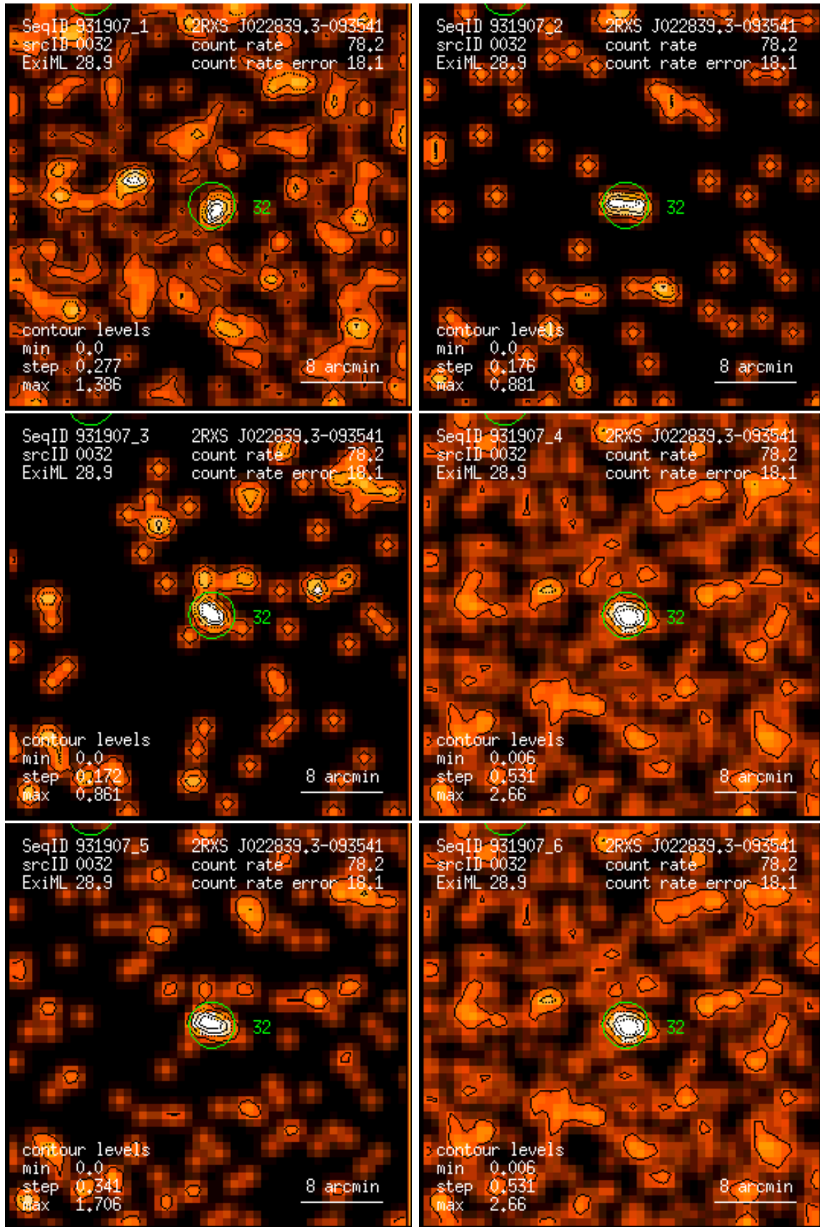
Figure 32: RASS 931907: detection 0032: band rate images, Gaussian filter: (1) PSPC channels 11 – 41, (2) 52 – 90, (3) 91 – 201, (4) 11 – 235, (5) 52 – 201, (6) 11 – 201. Broad band rates in counts/ks. Band rate contour levels in counts/ks/arcmin 2 .
