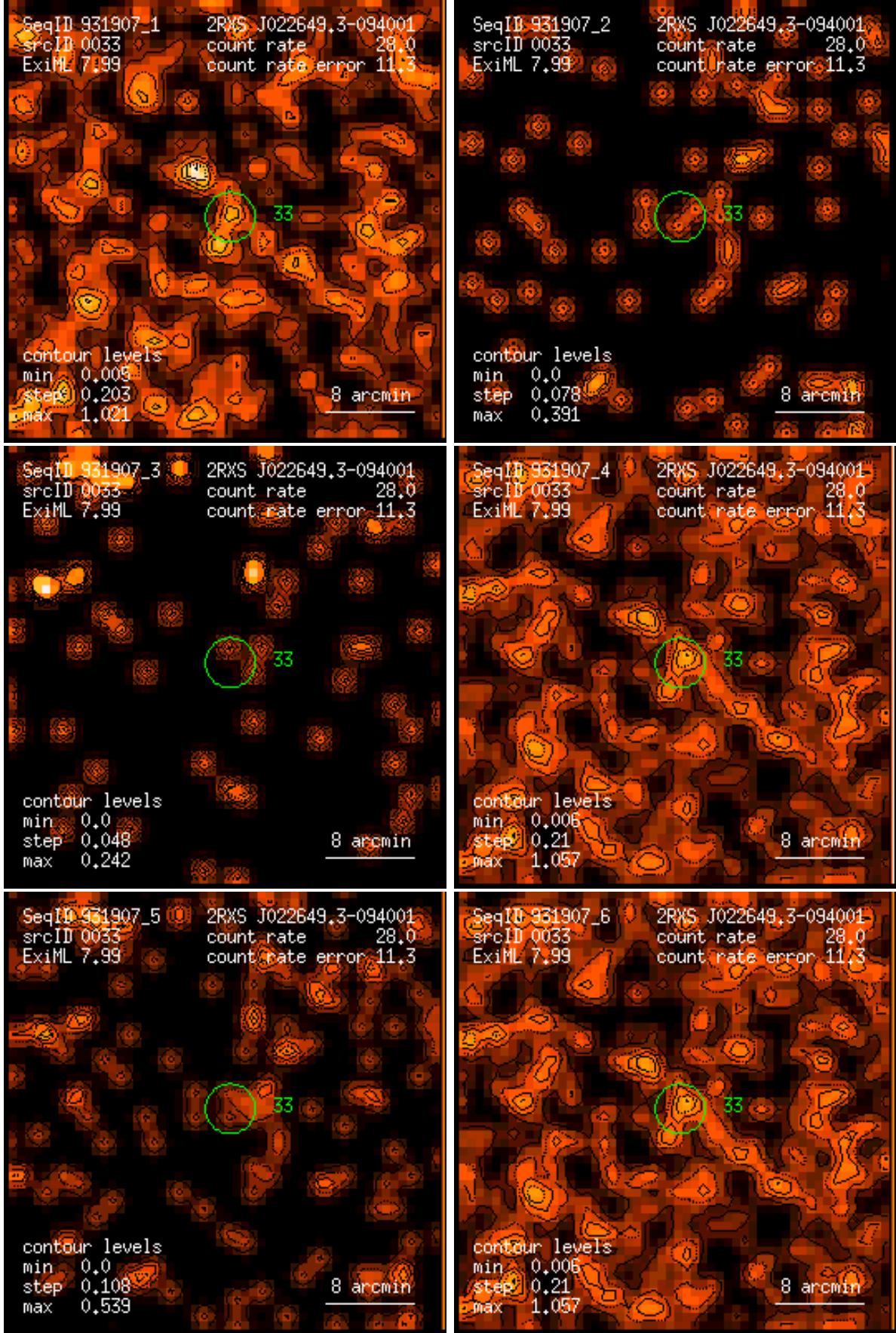
Figure 33: RASS 931907: detection 0033: band rate images, Gaussian filter: (1) PSPC channels 11 – 41, (2) 52 – 90, (3) 91 – 201, (4) 11 – 235, (5) 52 – 201, (6) 11 – 201. Broad band rates in counts/ks. Band rate contour levels in counts/ks/arcmin 2 .
