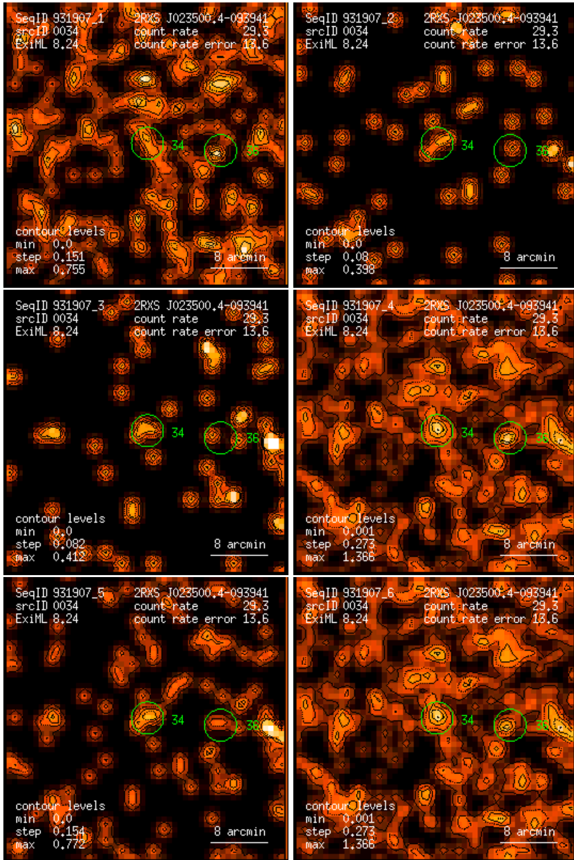
Figure 34: RASS 931907: detection 0034: band rate images, Gaussian filter: (1) PSPC channels 11 – 41, (2) 52 – 90, (3) 91 – 201, (4) 11 – 235, (5) 52 – 201, (6) 11 – 201. Broad band rates in counts/ks. Band rate contour levels in counts/ks/arcmin 2 .
