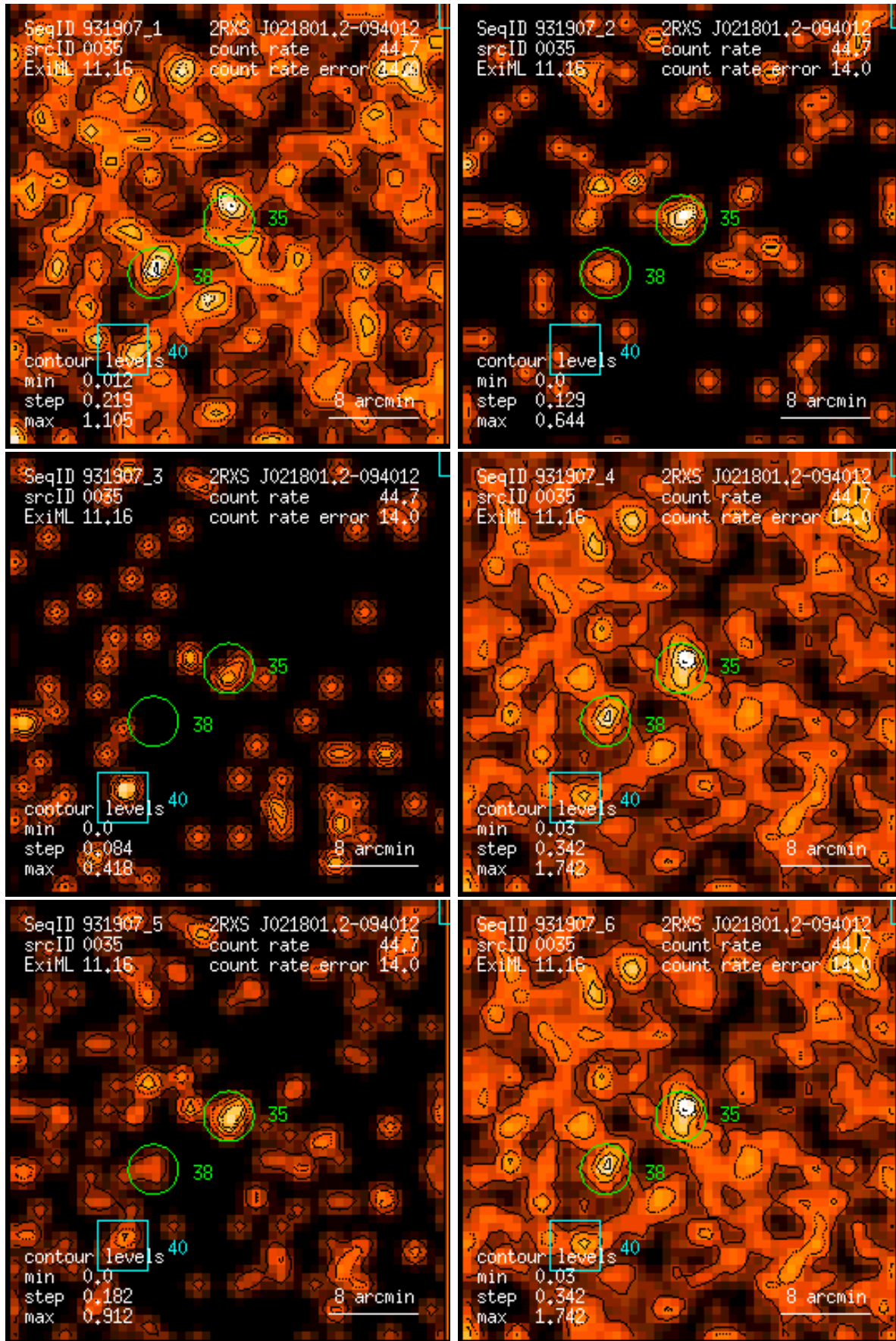
Figure 35: RASS 931907: detection 0035: band rate images, Gaussian filter: (1) PSPC channels 11 – 41, (2) 52 – 90, (3) 91 – 201, (4) 11 – 235, (5) 52 – 201, (6) 11 – 201. Broad band rates in counts/ks. Band rate contour levels in counts/ks/arcmin 2 .
