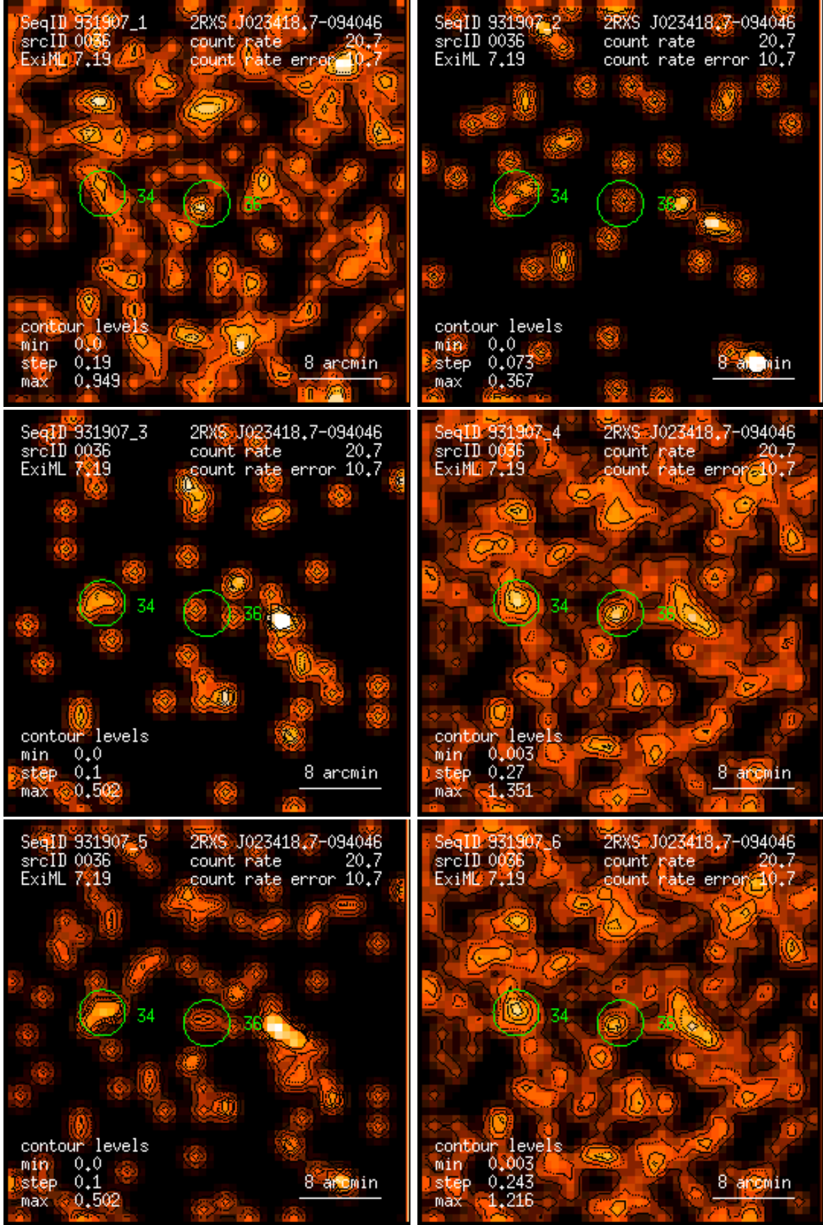
Figure 36: RASS 931907: detection 0036: band rate images, Gaussian filter: (1) PSPC channels 11 – 41, (2) 52 – 90, (3) 91 – 201, (4) 11 – 235, (5) 52 – 201, (6) 11 – 201. Broad band rates in counts/ks. Band rate contour levels in counts/ks/arcmin 2 .
