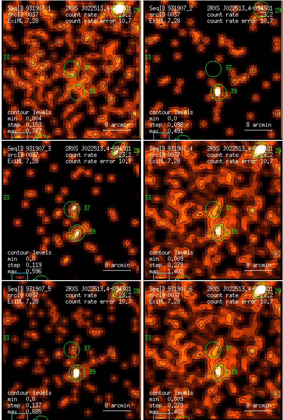
Figure 37: RASS 931907: detection 0037: band rate images, Gaussian filter: (1) PSPC channels 11 – 41, (2) 52 – 90, (3) 91 – 201, (4) 11 – 235, (5) 52 – 201, (6) 11 – 201. Broad band rates in counts/ks. Band rate contour levels in counts/ks/arcmin 2 .
