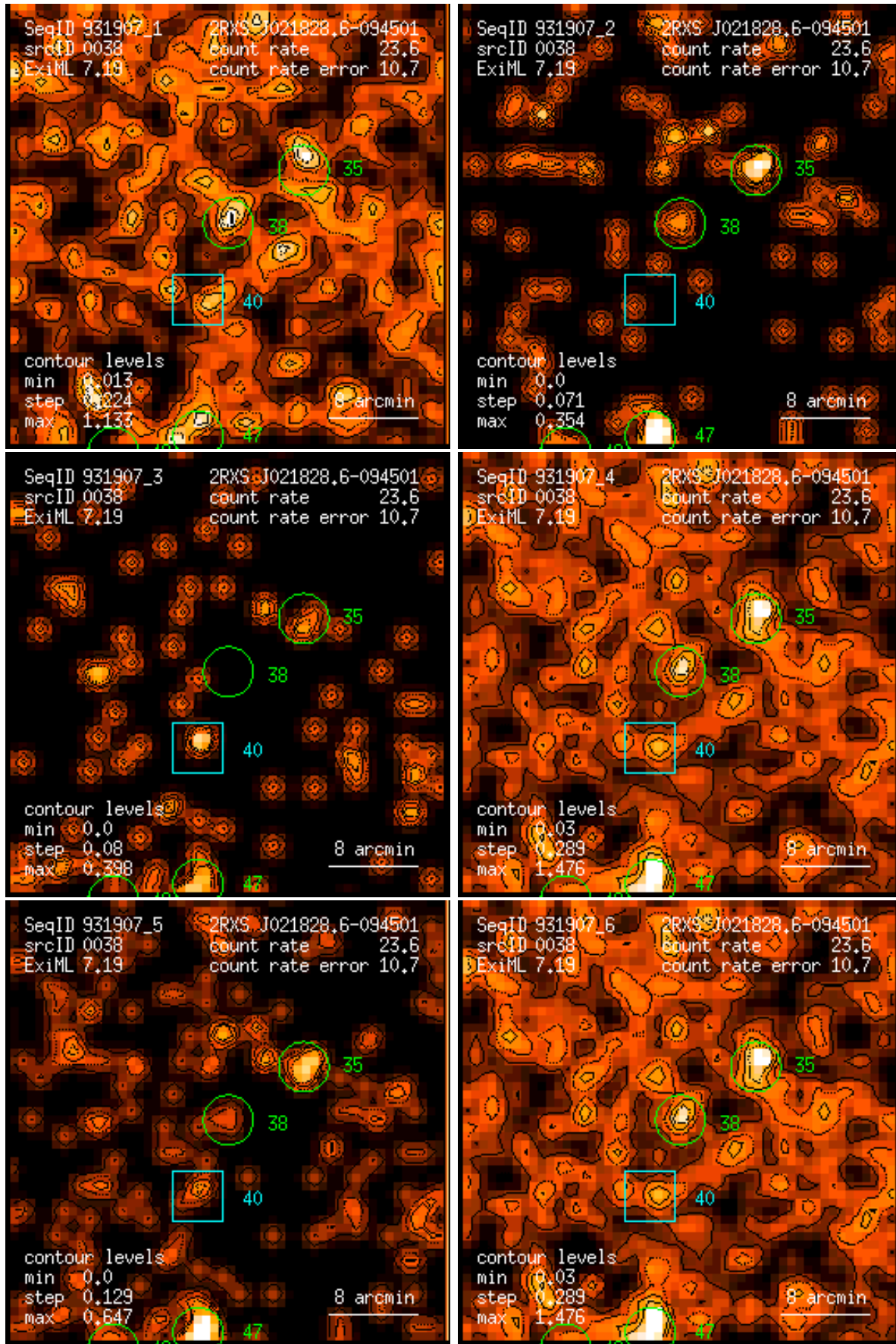
Figure 38: RASS 931907: detection 0038: band rate images, Gaussian filter: (1) PSPC channels 11 – 41, (2) 52 – 90, (3) 91 – 201, (4) 11 – 235, (5) 52 – 201, (6) 11 – 201. Broad band rates in counts/ks. Band rate contour levels in counts/ks/arcmin 2 .
