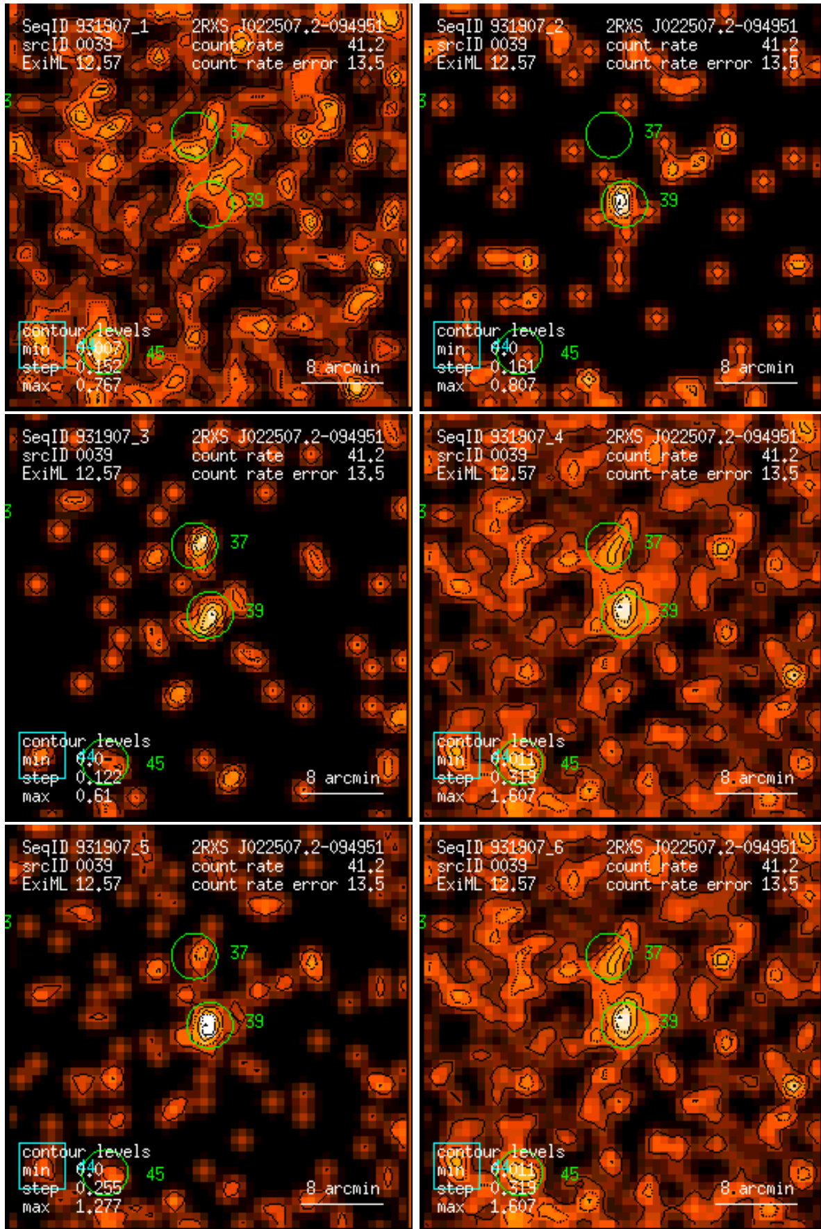
Figure 39: RASS 931907: detection 0039: band rate images, Gaussian filter: (1) PSPC channels 11 – 41, (2) 52 – 90, (3) 91 – 201, (4) 11 – 235, (5) 52 – 201, (6) 11 – 201. Broad band rates in counts/ks. Band rate contour levels in counts/ks/arcmin 2 .
