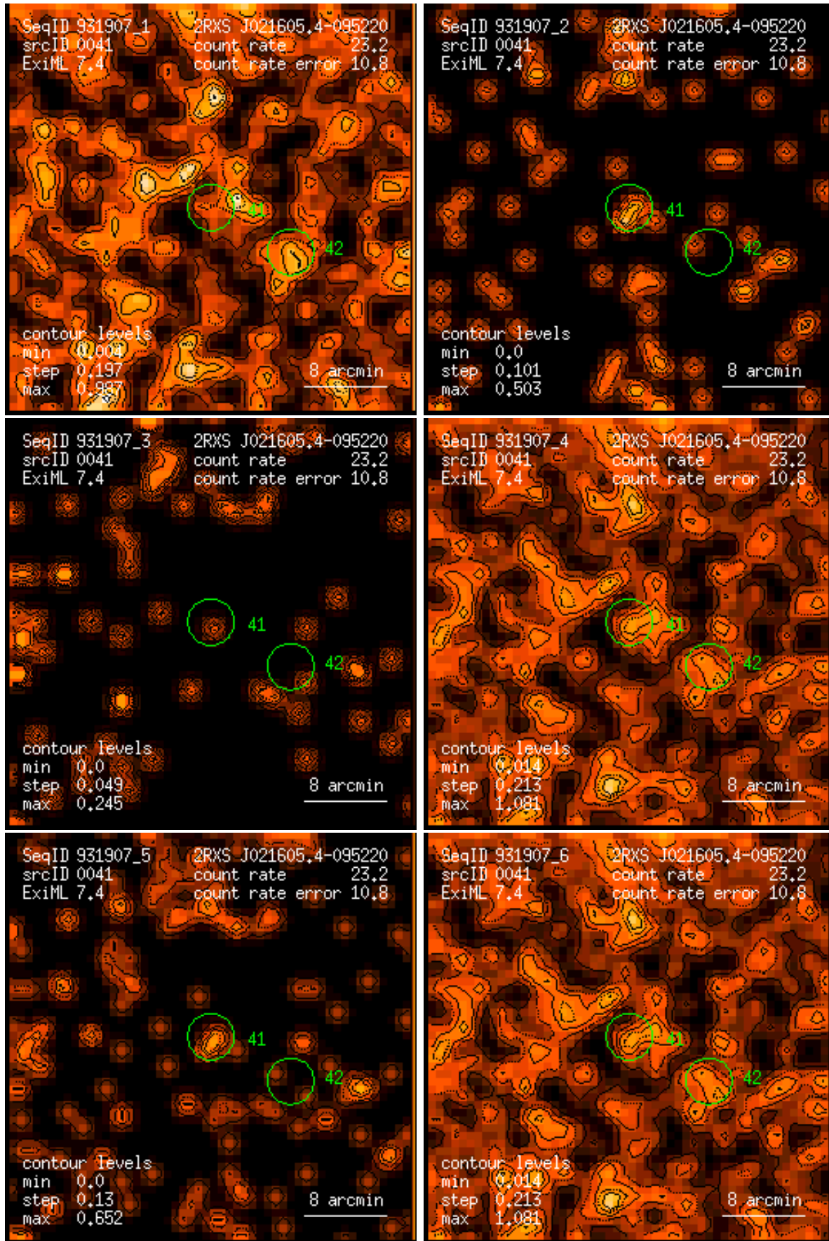
Figure 41: RASS 931907: detection 0041: band rate images, Gaussian filter: (1) PSPC channels 11 – 41, (2) 52 – 90, (3) 91 – 201, (4) 11 – 235, (5) 52 – 201, (6) 11 – 201. Broad band rates in counts/ks. Band rate contour levels in counts/ks/arcmin 2 .
