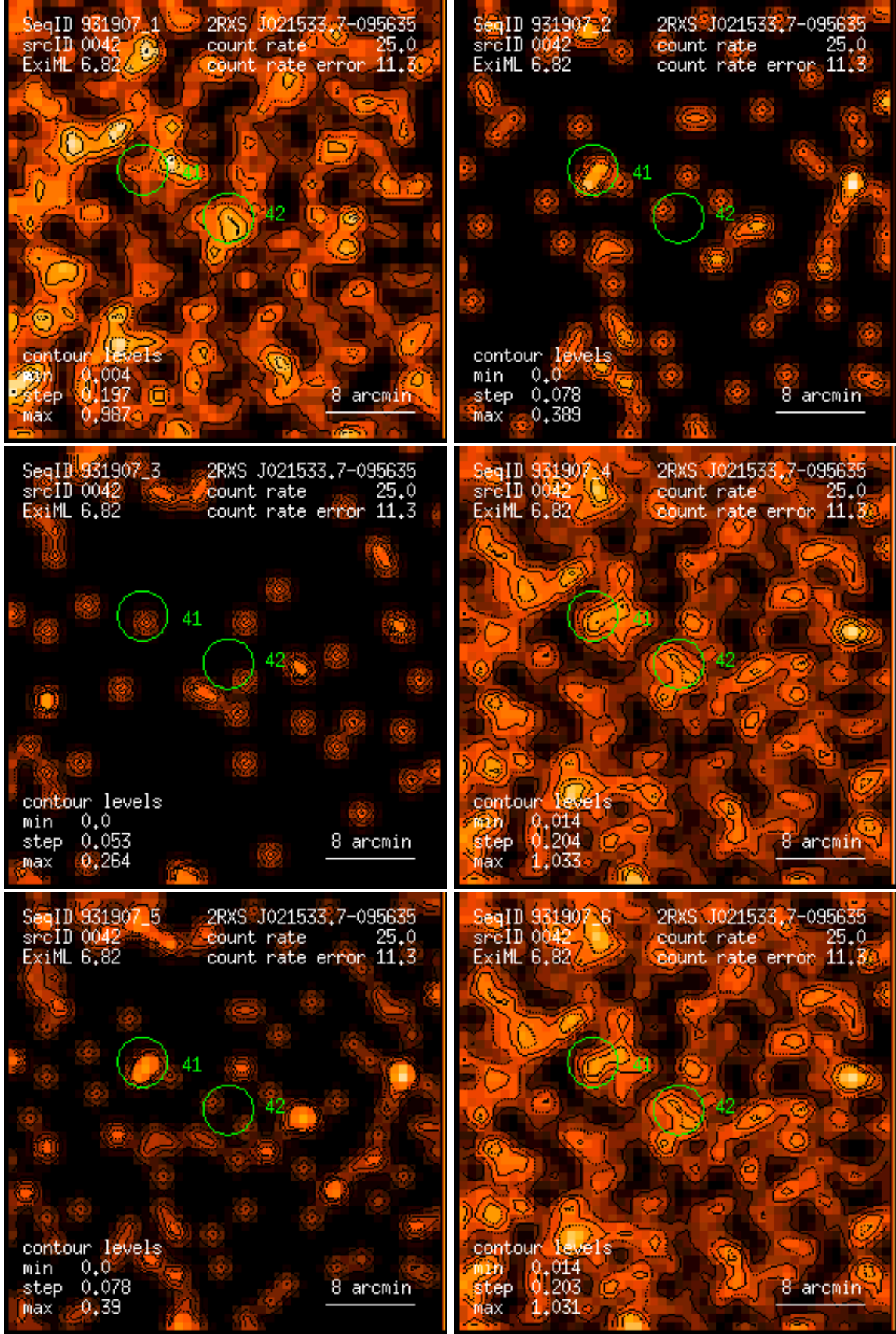
Figure 42: RASS 931907: detection 0042: band rate images, Gaussian filter: (1) PSPC channels 11 – 41, (2) 52 – 90, (3) 91 – 201, (4) 11 – 235, (5) 52 – 201, (6) 11 – 201. Broad band rates in counts/ks. Band rate contour levels in counts/ks/arcmin 2 .
