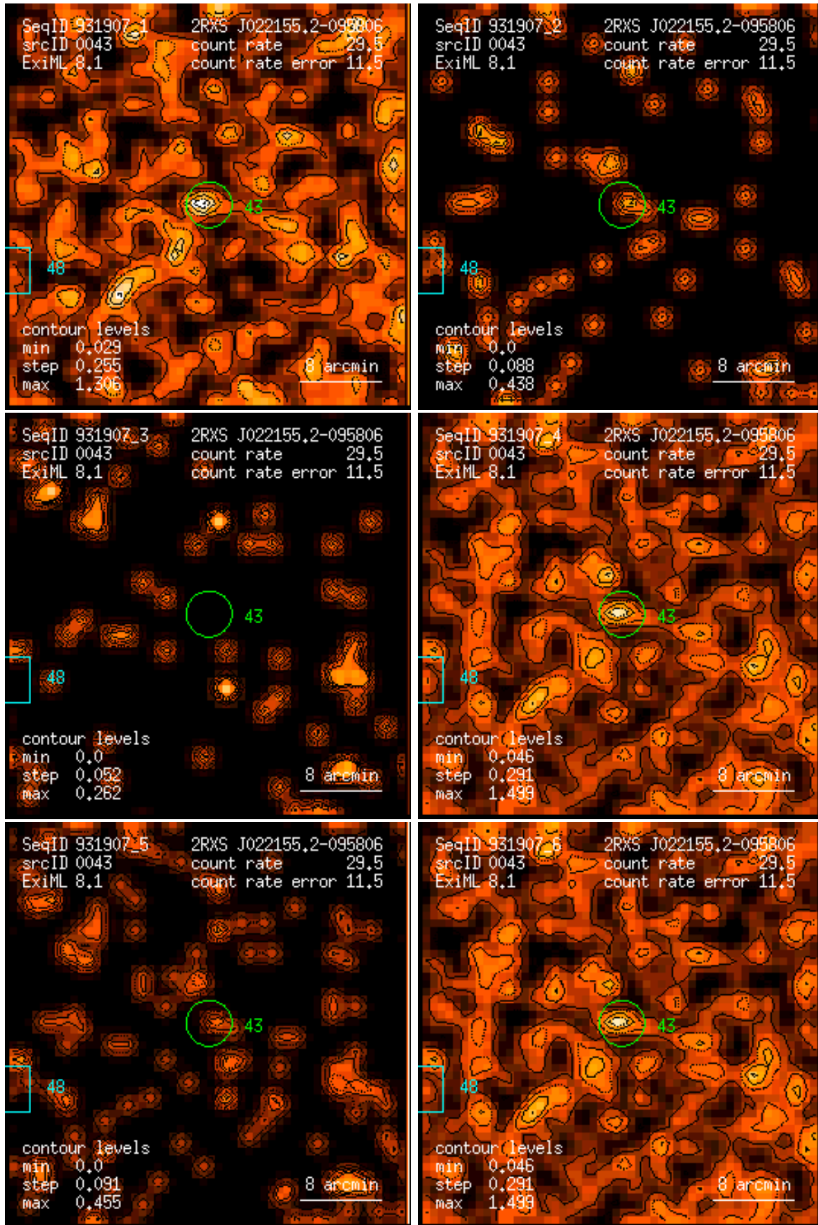
Figure 43: RASS 931907: detection 0043: band rate images, Gaussian filter: (1) PSPC channels 11 – 41, (2) 52 – 90, (3) 91 – 201, (4) 11 – 235, (5) 52 – 201, (6) 11 – 201. Broad band rates in counts/ks. Band rate contour levels in counts/ks/arcmin 2 .
