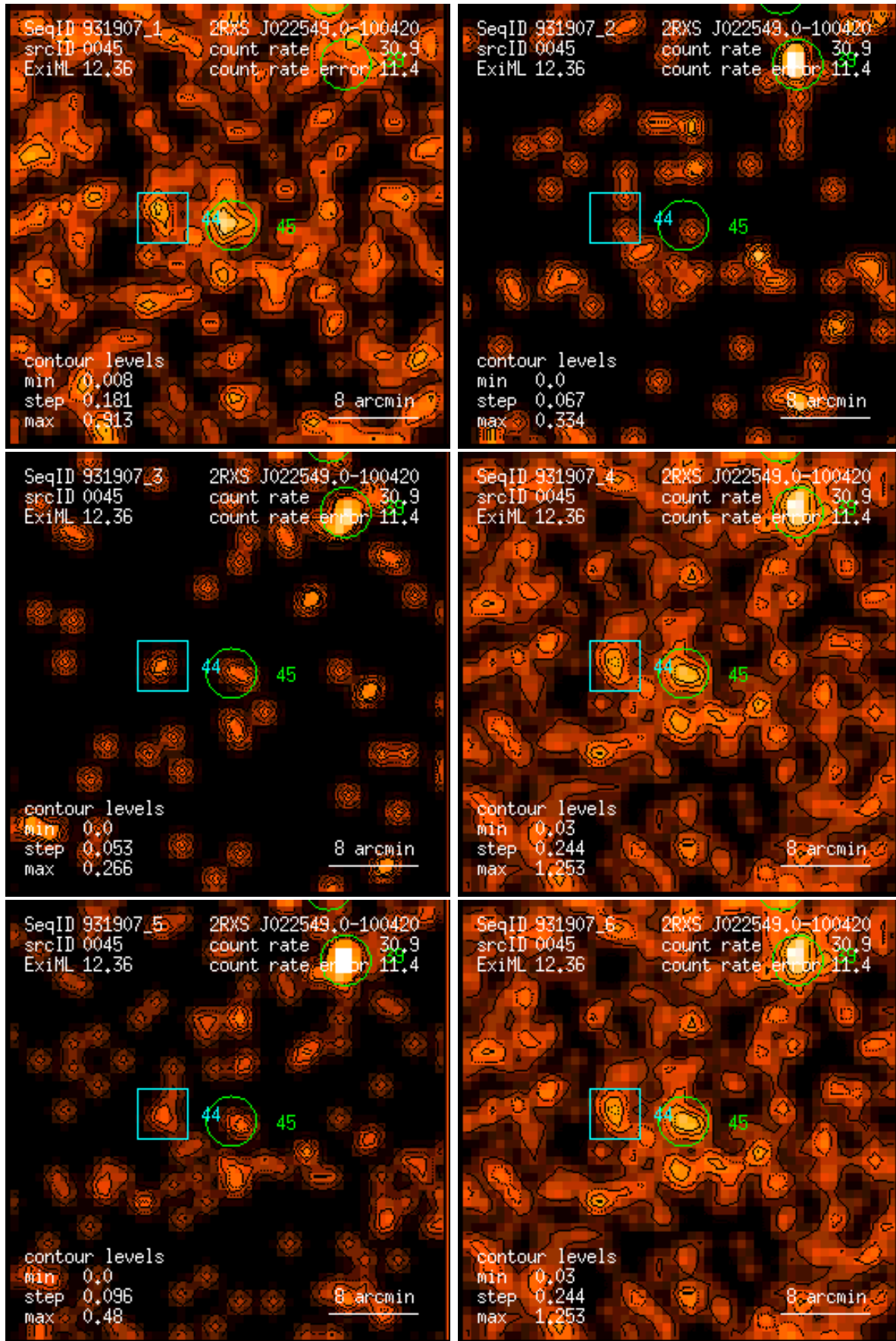
Figure 45: RASS 931907: detection 0045: band rate images, Gaussian filter: (1) PSPC channels 11 – 41, (2) 52 – 90, (3) 91 – 201, (4) 11 – 235, (5) 52 – 201, (6) 11 – 201. Broad band rates in counts/ks. Band rate contour levels in counts/ks/arcmin 2 .
