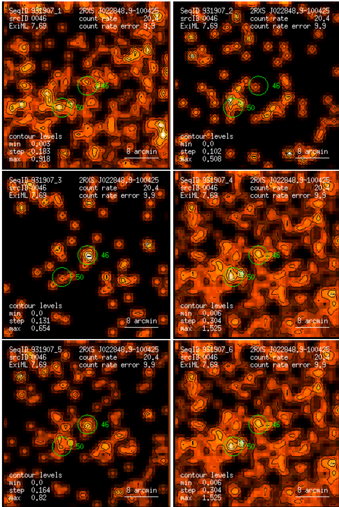
Figure 46: RASS 931907: detection 0046: band rate images, Gaussian filter: (1) PSPC channels 11 – 41, (2) 52 – 90, (3) 91 – 201, (4) 11 – 235, (5) 52 – 201, (6) 11 – 201. Broad band rates in counts/ks. Band rate contour levels in counts/ks/arcmin 2 .
