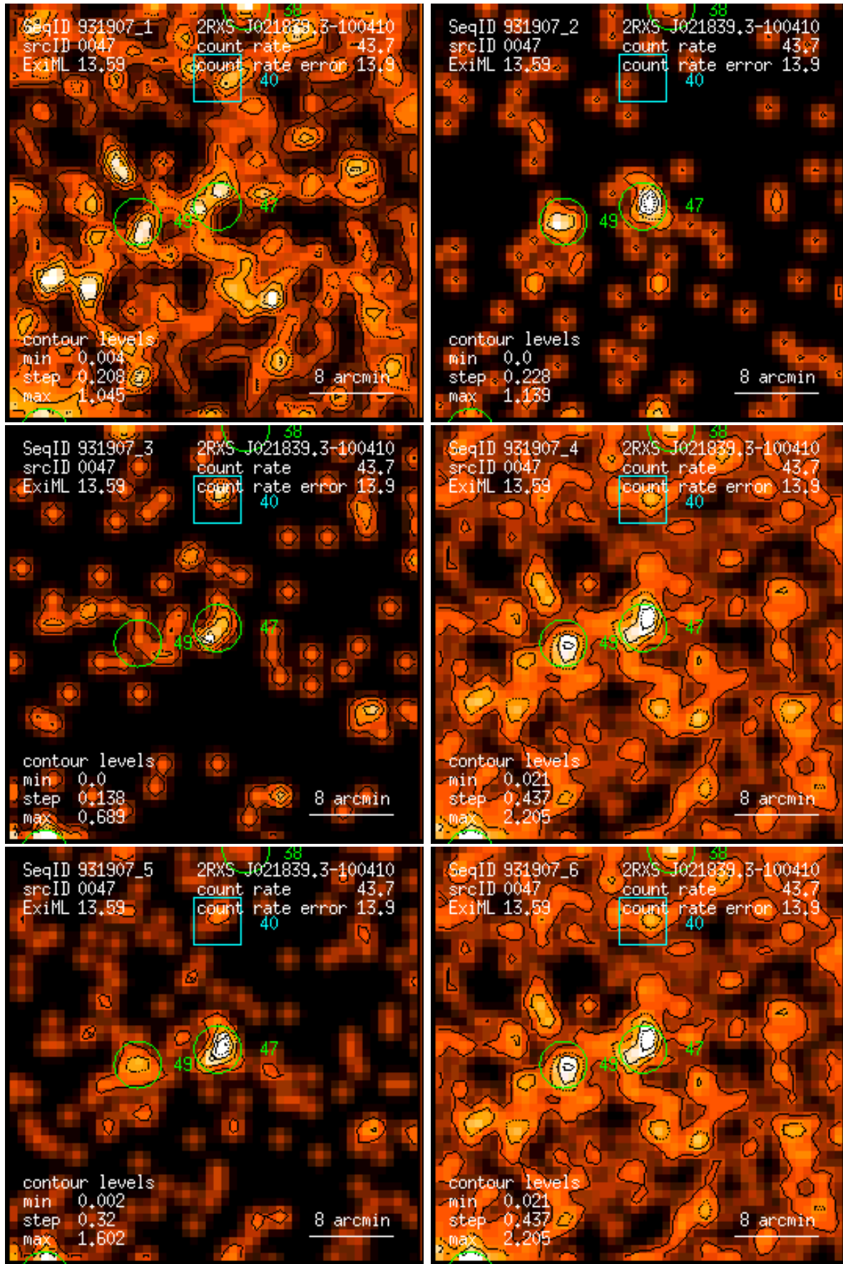
Figure 47: RASS 931907: detection 0047: band rate images, Gaussian filter: (1) PSPC channels 11 – 41, (2) 52 – 90, (3) 91 – 201, (4) 11 – 235, (5) 52 – 201, (6) 11 – 201. Broad band rates in counts/ks. Band rate contour levels in counts/ks/arcmin 2 .
