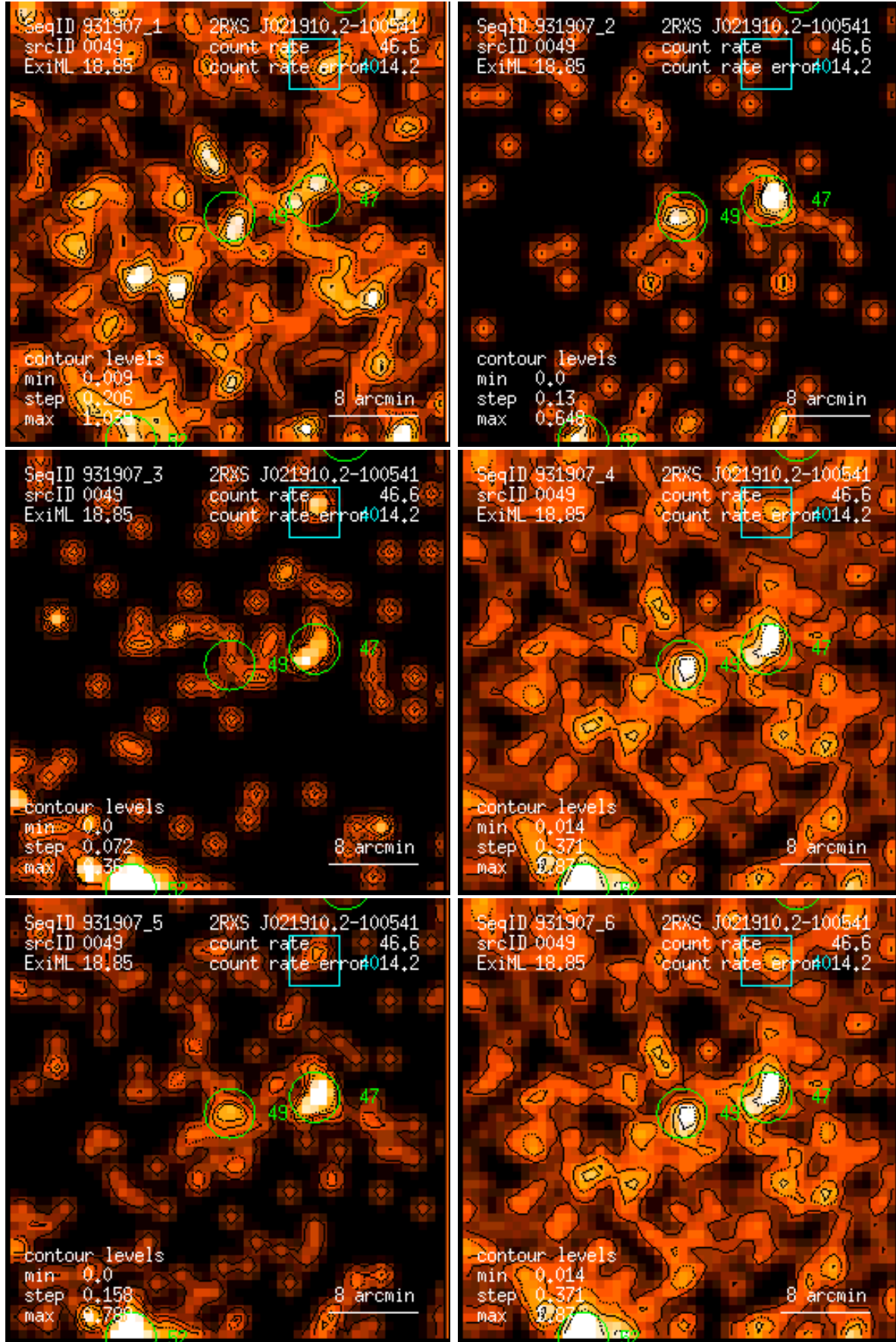
Figure 49: RASS 931907: detection 0049: band rate images, Gaussian filter: (1) PSPC channels 11 – 41, (2) 52 – 90, (3) 91 – 201, (4) 11 – 235, (5) 52 – 201, (6) 11 – 201. Broad band rates in counts/ks. Band rate contour levels in counts/ks/arcmin 2 .
