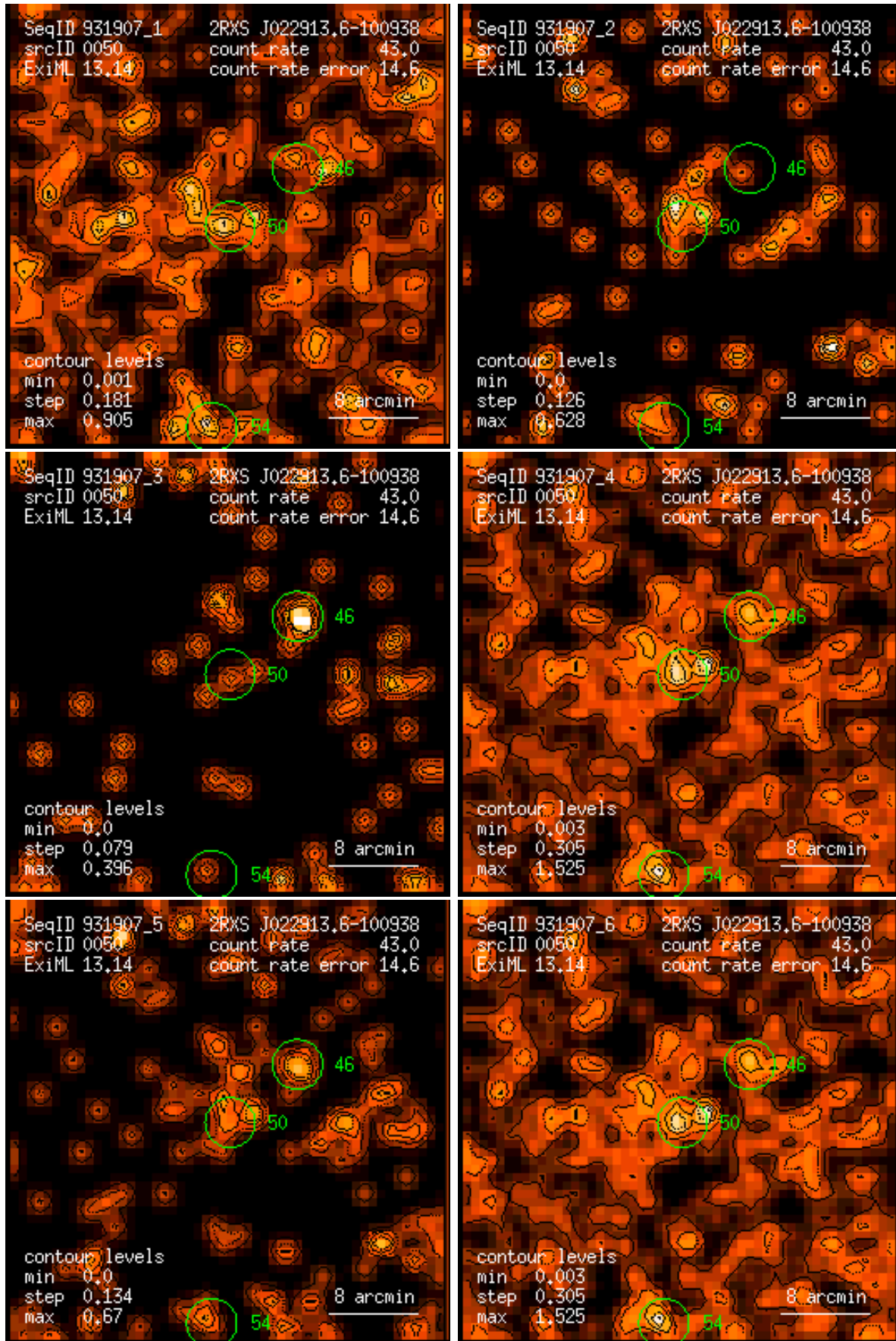
Figure 50: RASS 931907: detection 0050: band rate images, Gaussian filter: (1) PSPC channels 11 – 41, (2) 52 – 90, (3) 91 – 201, (4) 11 – 235, (5) 52 – 201, (6) 11 – 201. Broad band rates in counts/ks. Band rate contour levels in counts/ks/arcmin 2 .
