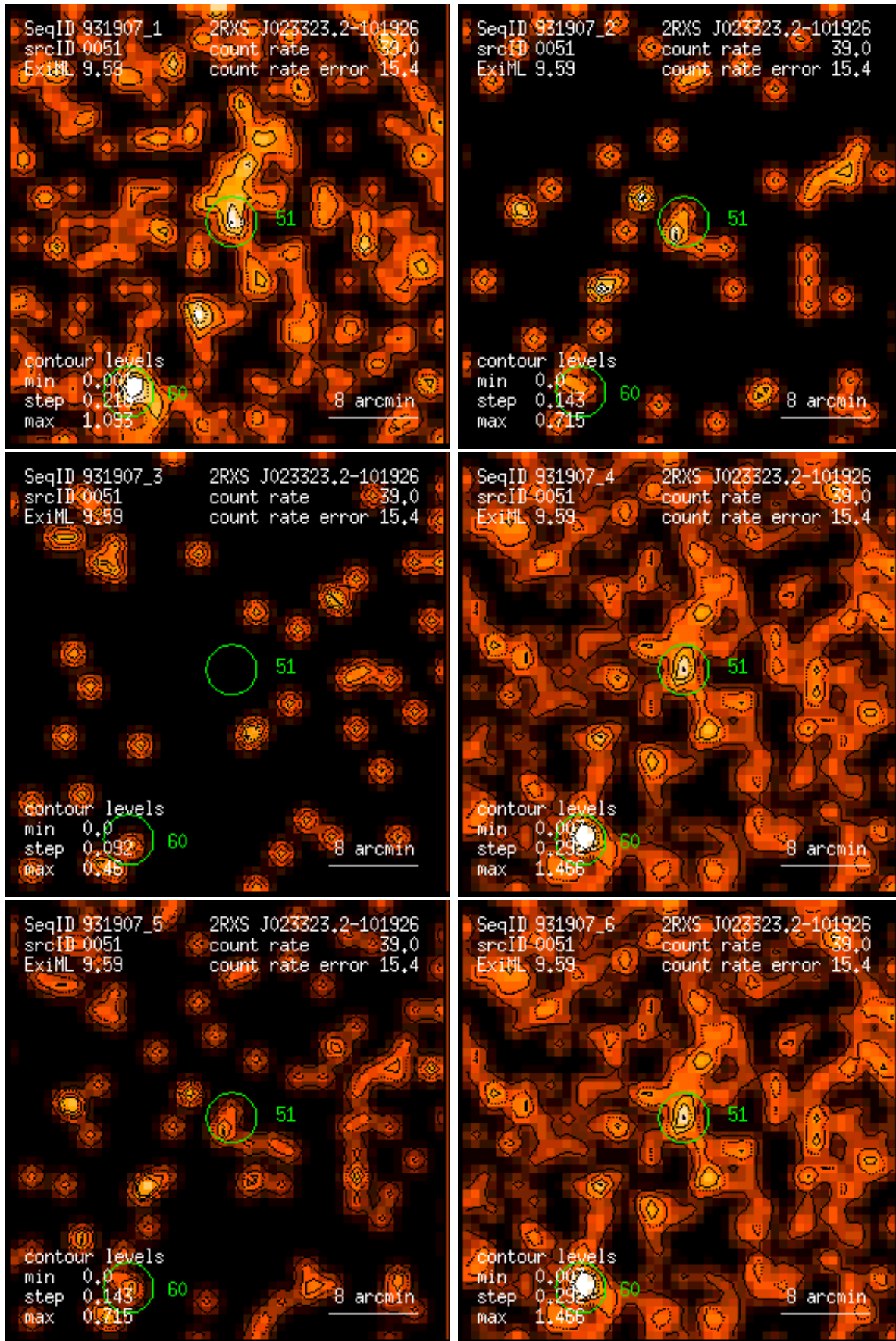
Figure 51: RASS 931907: detection 0051: band rate images, Gaussian filter: (1) PSPC channels 11 – 41, (2) 52 – 90, (3) 91 – 201, (4) 11 – 235, (5) 52 – 201, (6) 11 – 201. Broad band rates in counts/ks. Band rate contour levels in counts/ks/arcmin 2 .
