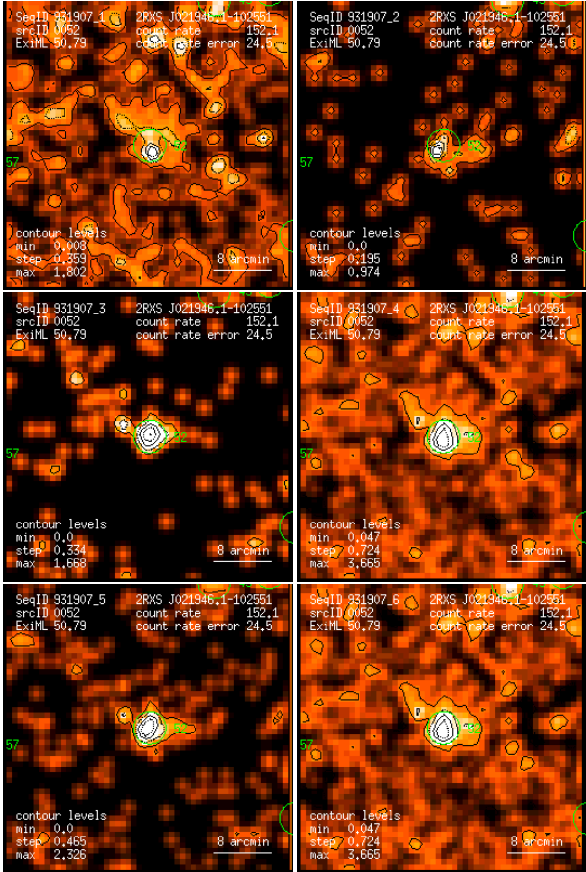
Figure 52: RASS 931907: detection 0052: band rate images, Gaussian filter: (1) PSPC channels 11 – 41, (2) 52 – 90, (3) 91 – 201, (4) 11 – 235, (5) 52 – 201, (6) 11 – 201. Broad band rates in counts/ks. Band rate contour levels in counts/ks/arcmin 2 .
