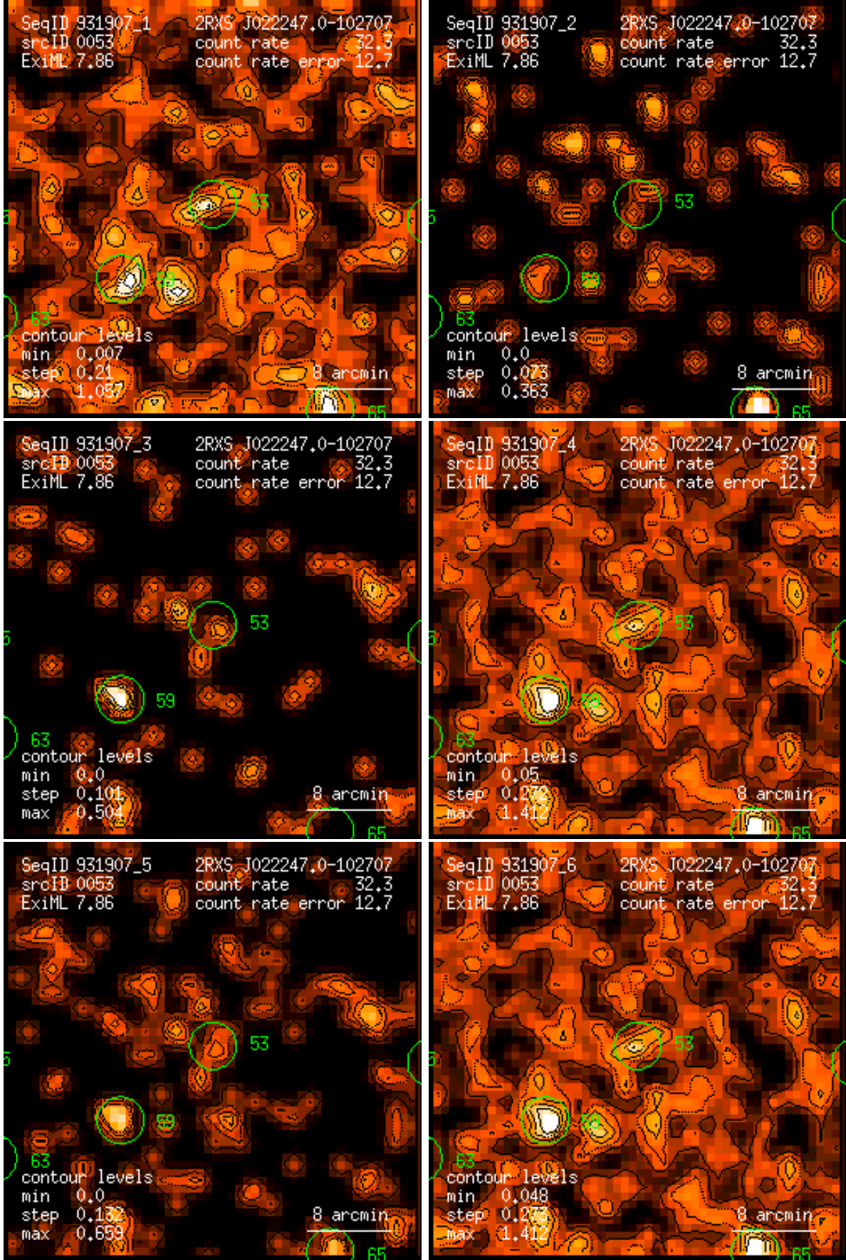
Figure 53: RASS 931907: detection 0053: band rate images, Gaussian filter: (1) PSPC channels 11 – 41, (2) 52 – 90, (3) 91 – 201, (4) 11 – 235, (5) 52 – 201, (6) 11 – 201. Broad band rates in counts/ks. Band rate contour levels in counts/ks/arcmin 2 .
