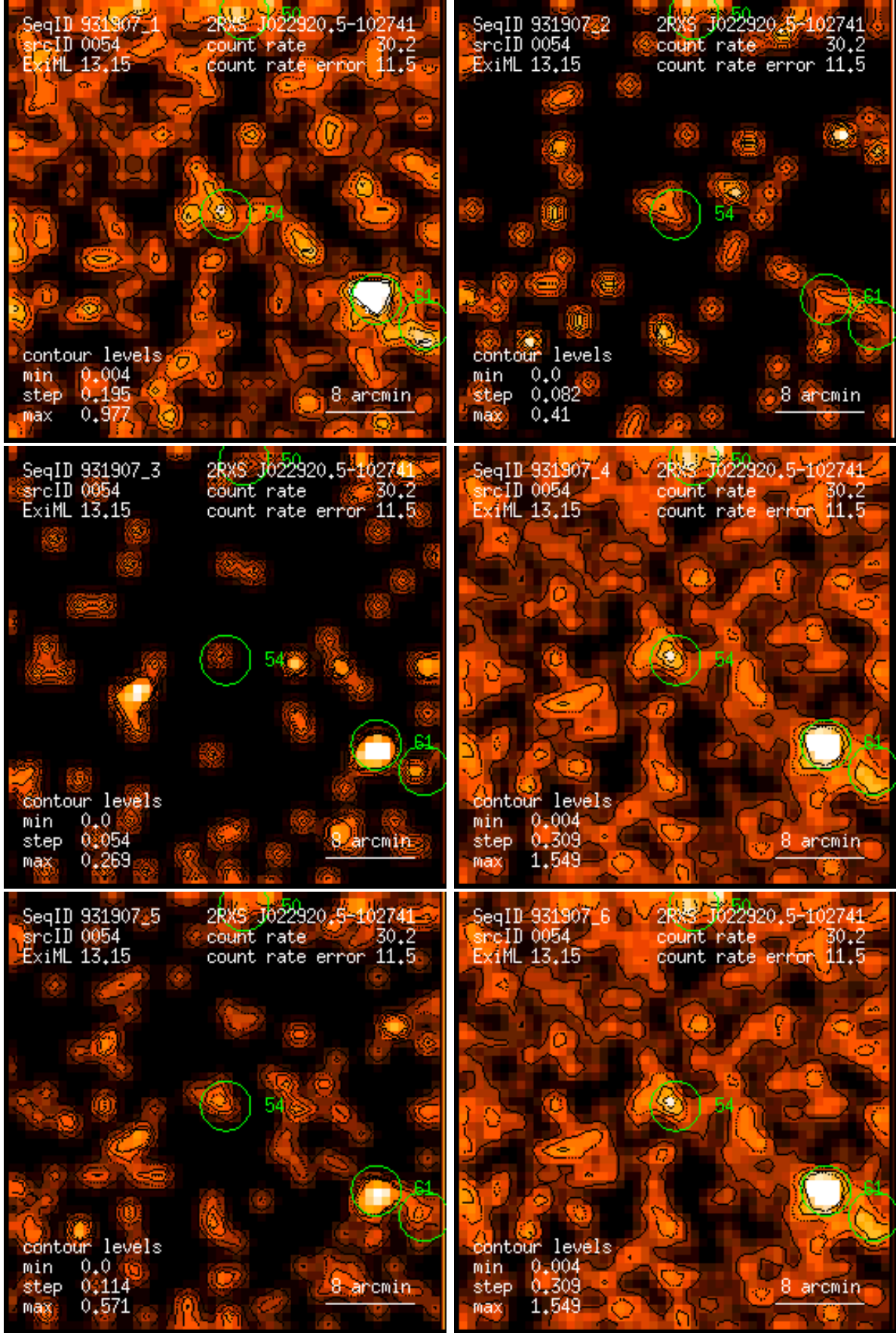
Figure 54: RASS 931907: detection 0054: band rate images, Gaussian filter: (1) PSPC channels 11 – 41, (2) 52 – 90, (3) 91 – 201, (4) 11 – 235, (5) 52 – 201, (6) 11 – 201. Broad band rates in counts/ks. Band rate contour levels in counts/ks/arcmin 2 .
