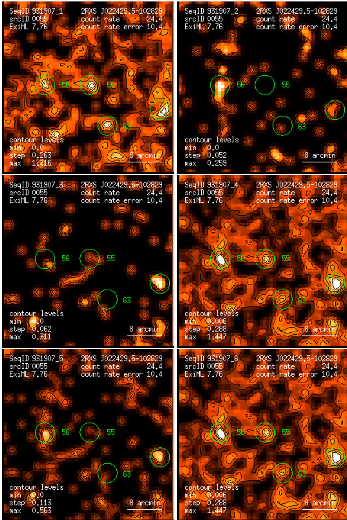
Figure 55: RASS 931907: detection 0055: band rate images, Gaussian filter: (1) PSPC channels 11 – 41, (2) 52 – 90, (3) 91 – 201, (4) 11 – 235, (5) 52 – 201, (6) 11 – 201. Broad band rates in counts/ks. Band rate contour levels in counts/ks/arcmin 2 .
