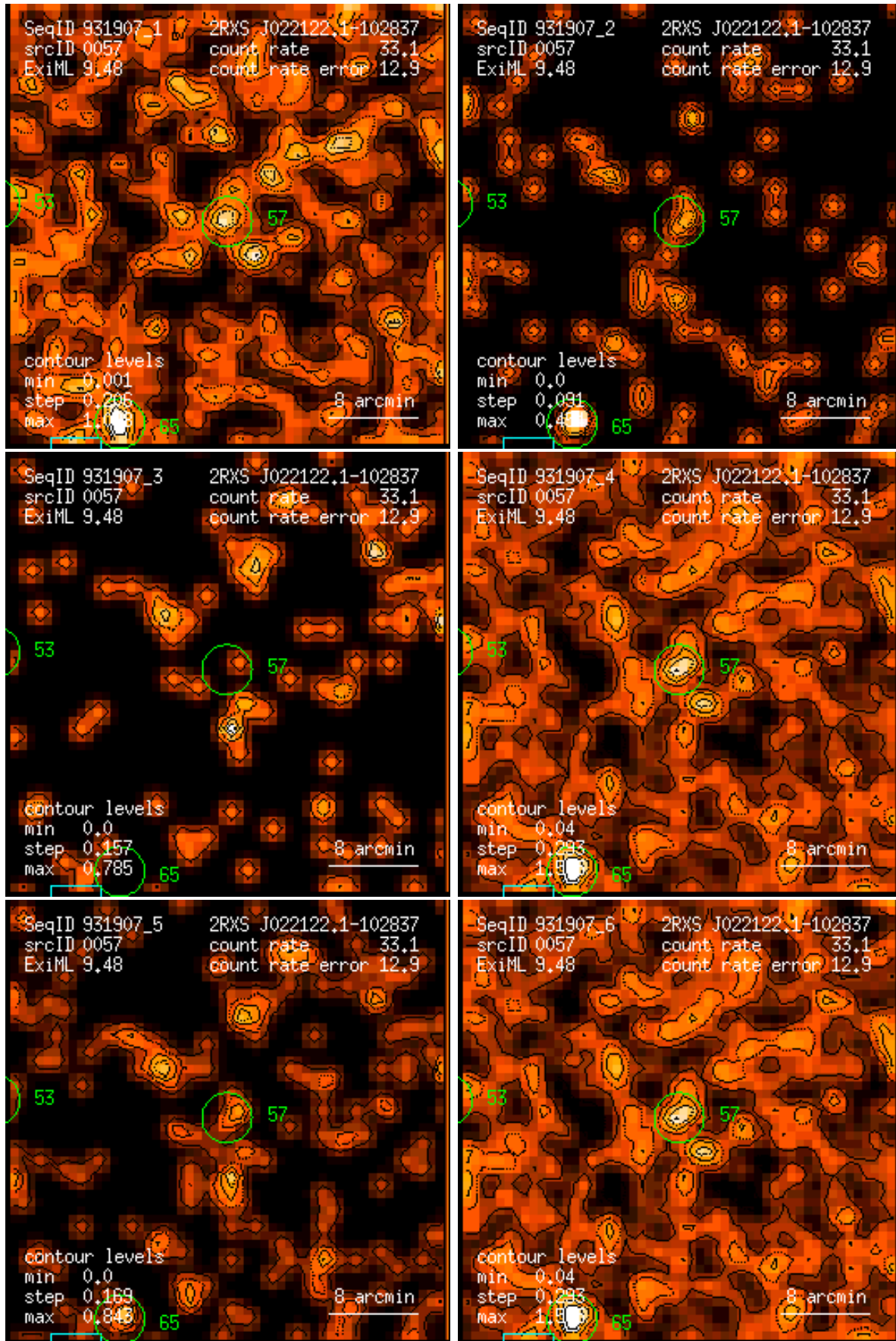
Figure 57: RASS 931907: detection 0057: band rate images, Gaussian filter: (1) PSPC channels 11 – 41, (2) 52 – 90, (3) 91 – 201, (4) 11 – 235, (5) 52 – 201, (6) 11 – 201. Broad band rates in counts/ks. Band rate contour levels in counts/ks/arcmin 2 .
