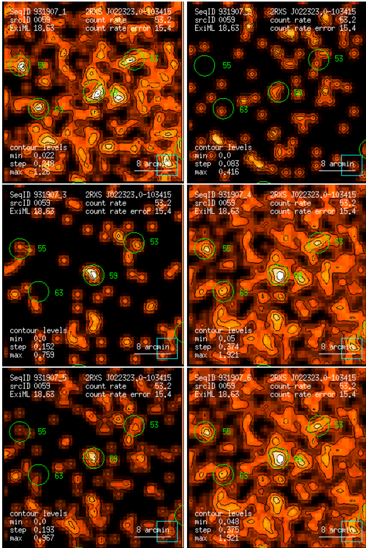
Figure 59: RASS 931907: detection 0059: band rate images, Gaussian filter: (1) PSPC channels 11 – 41, (2) 52 – 90, (3) 91 – 201, (4) 11 – 235, (5) 52 – 201, (6) 11 – 201. Broad band rates in counts/ks. Band rate contour levels in counts/ks/arcmin 2 .
