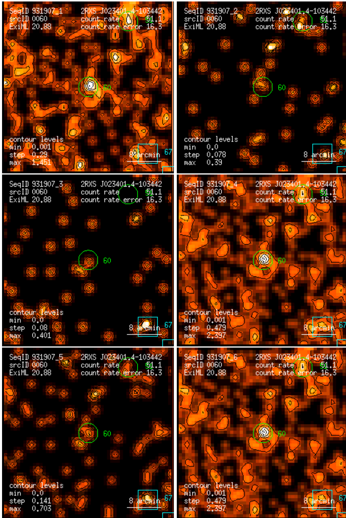
Figure 60: RASS 931907: detection 0060: band rate images, Gaussian filter: (1) PSPC channels 11 – 41, (2) 52 – 90, (3) 91 – 201, (4) 11 – 235, (5) 52 – 201, (6) 11 – 201. Broad band rates in counts/ks. Band rate contour levels in counts/ks/arcmin 2 .
