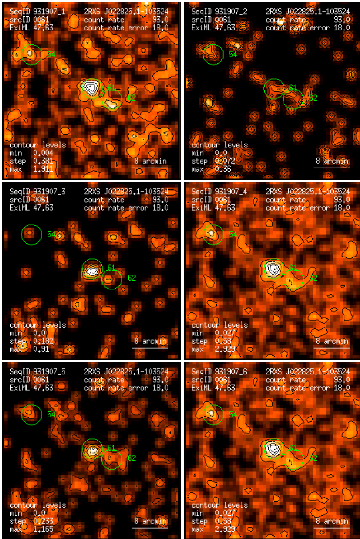
Figure 61: RASS 931907: detection 0061: band rate images, Gaussian filter: (1) PSPC channels 11 – 41, (2) 52 – 90, (3) 91 – 201, (4) 11 – 235, (5) 52 – 201, (6) 11 – 201. Broad band rates in counts/ks. Band rate contour levels in counts/ks/arcmin 2 .
