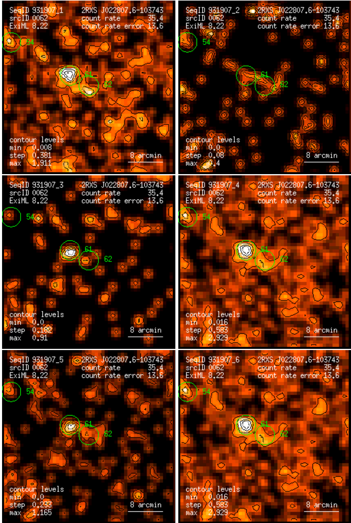
Figure 62: RASS 931907: detection 0062: band rate images, Gaussian filter: (1) PSPC channels 11 – 41, (2) 52 – 90, (3) 91 – 201, (4) 11 – 235, (5) 52 – 201, (6) 11 – 201. Broad band rates in counts/ks. Band rate contour levels in counts/ks/arcmin 2 .
