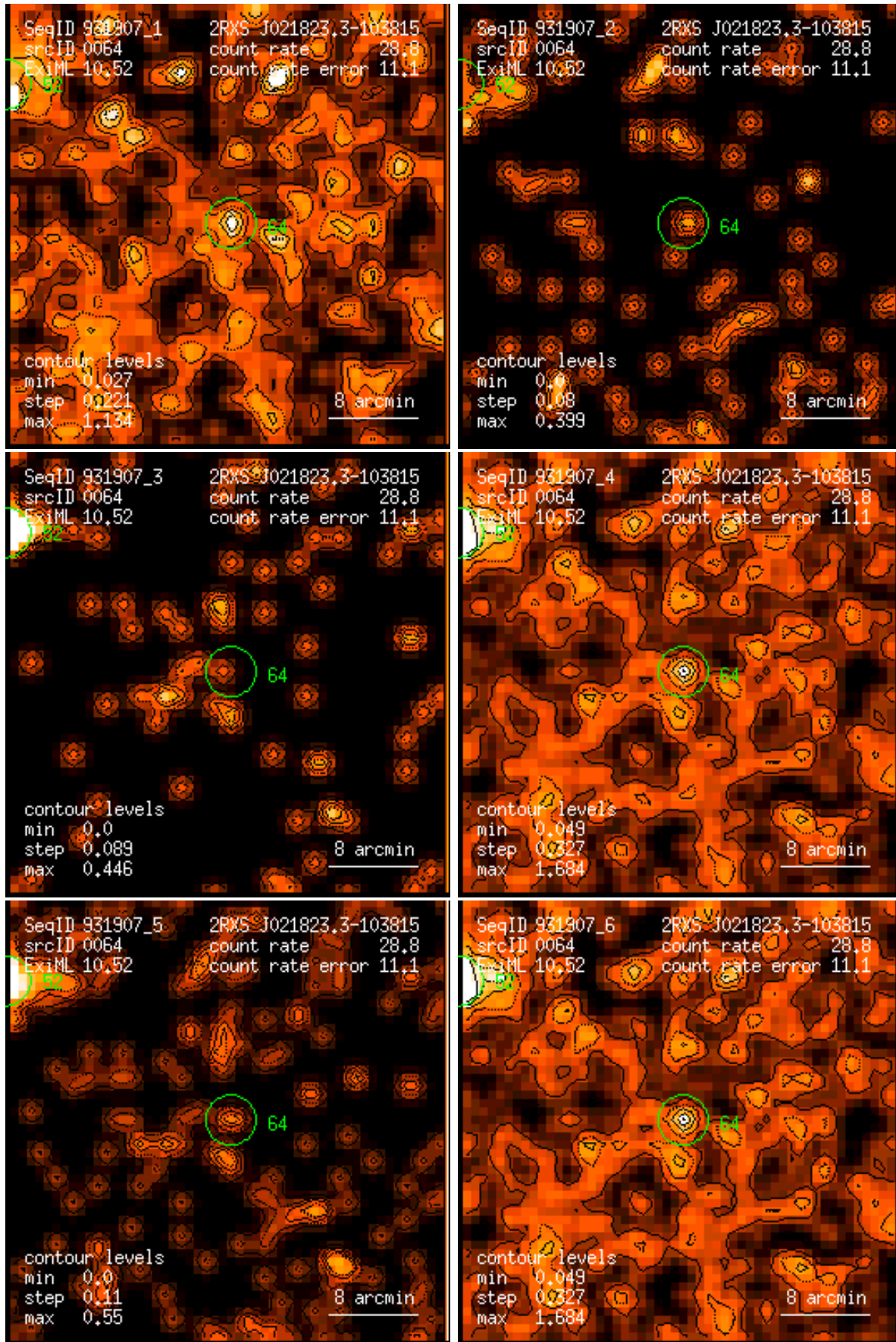
Figure 64: RASS 931907: detection 0064: band rate images, Gaussian filter: (1) PSPC channels 11 – 41, (2) 52 – 90, (3) 91 – 201, (4) 11 – 235, (5) 52 – 201, (6) 11 – 201. Broad band rates in counts/ks. Band rate contour levels in counts/ks/arcmin 2 .
