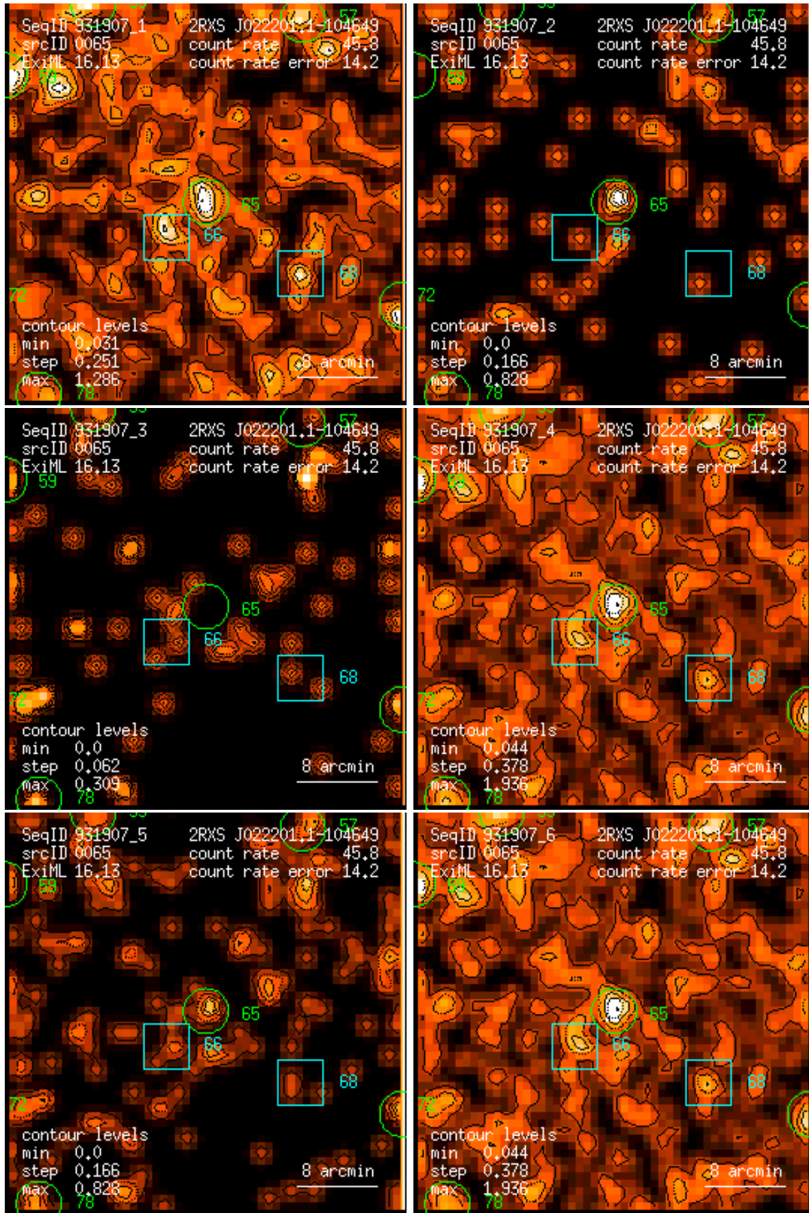
Figure 65: RASS 931907: detection 0065: band rate images, Gaussian filter: (1) PSPC channels 11 – 41, (2) 52 – 90, (3) 91 – 201, (4) 11 – 235, (5) 52 – 201, (6) 11 – 201. Broad band rates in counts/ks. Band rate contour levels in counts/ks/arcmin 2 .
