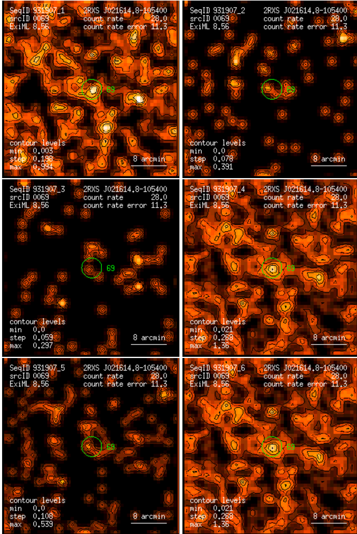
Figure 69: RASS 931907: detection 0069: band rate images, Gaussian filter: (1) PSPC channels 11 – 41, (2) 52 – 90, (3) 91 – 201, (4) 11 – 235, (5) 52 – 201, (6) 11 – 201. Broad band rates in counts/ks. Band rate contour levels in counts/ks/arcmin 2 .
