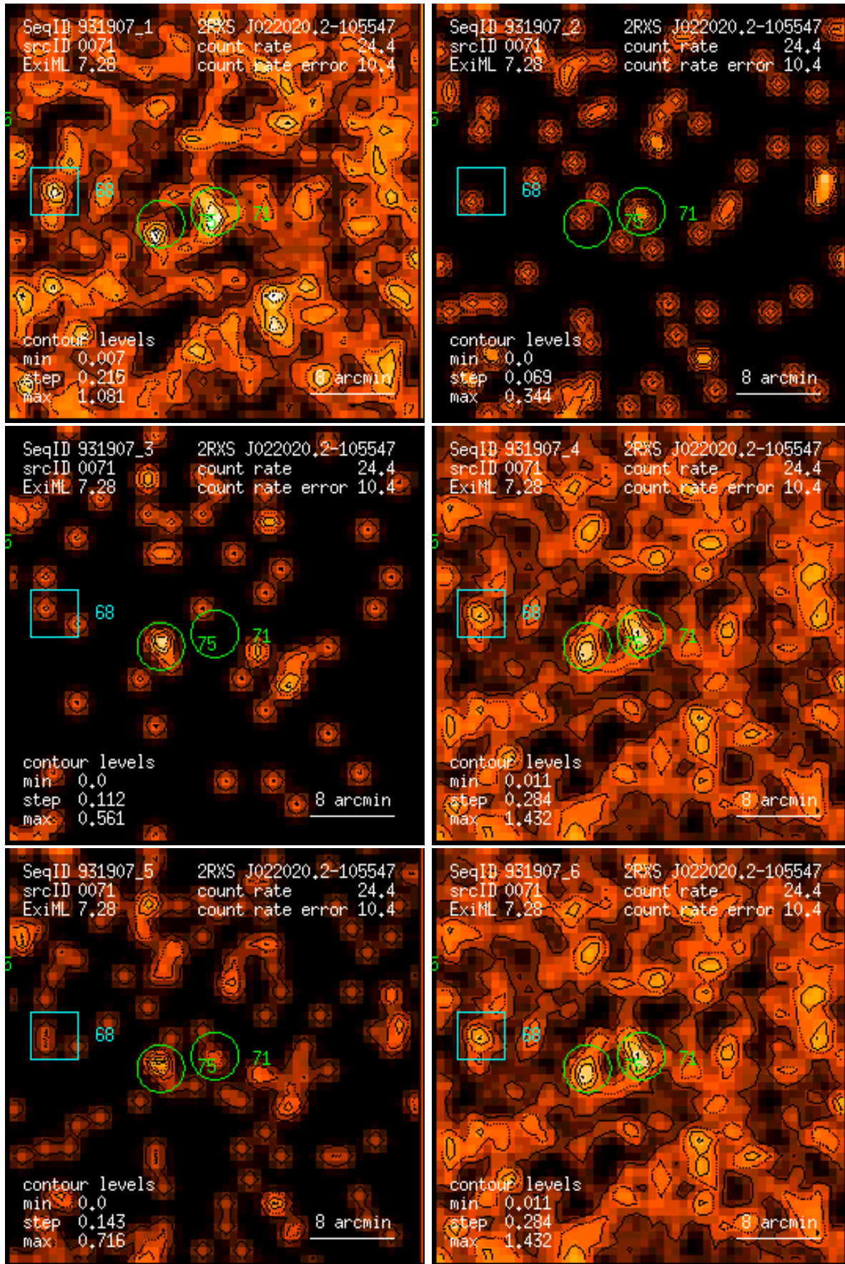
Figure 71: RASS 931907: detection 0071: band rate images, Gaussian filter: (1) PSPC channels 11 – 41, (2) 52 – 90, (3) 91 – 201, (4) 11 – 235, (5) 52 – 201, (6) 11 – 201. Broad band rates in counts/ks. Band rate contour levels in counts/ks/arcmin 2 .
