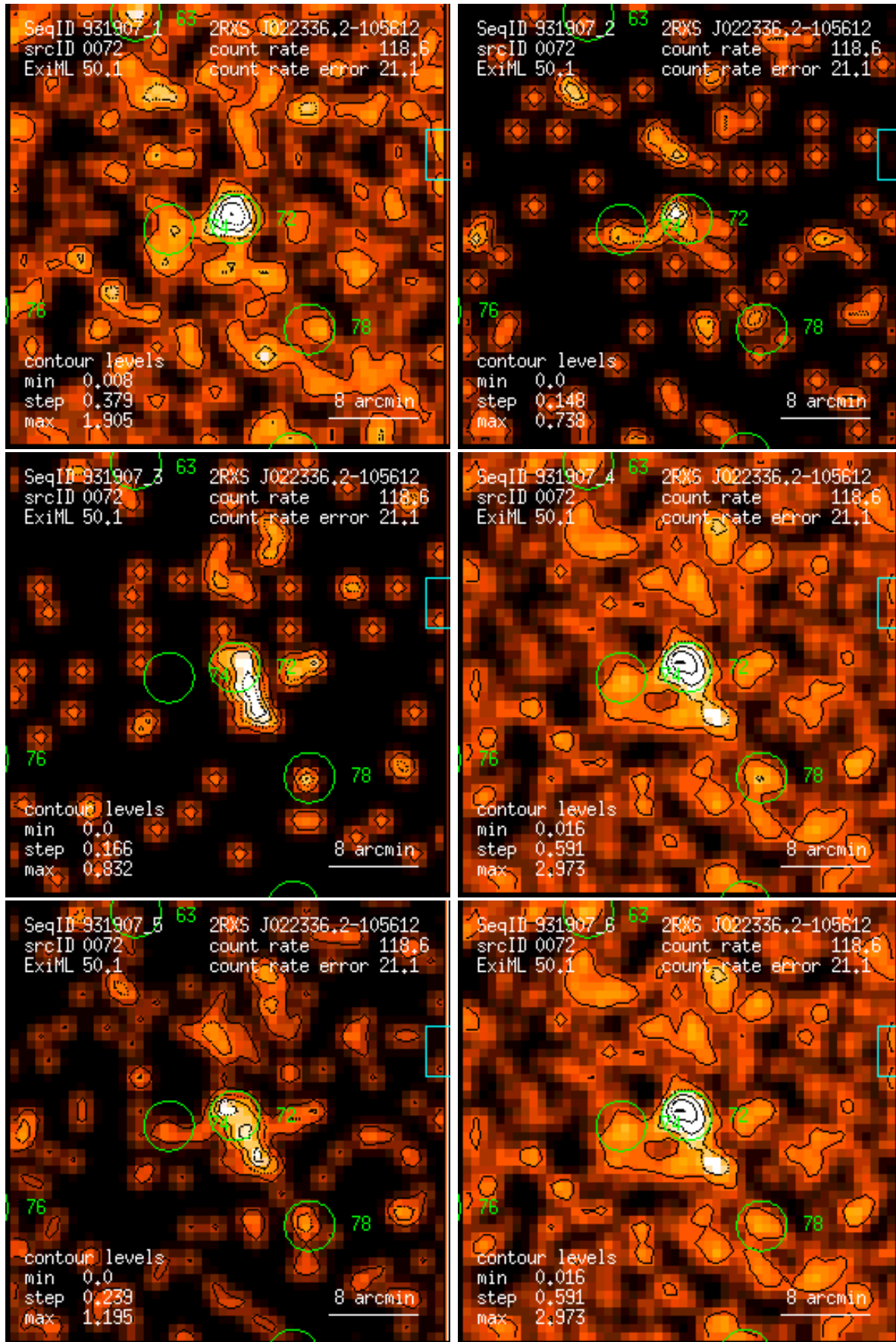
Figure 72: RASS 931907: detection 0072: band rate images, Gaussian filter: (1) PSPC channels 11 – 41, (2) 52 – 90, (3) 91 – 201, (4) 11 – 235, (5) 52 – 201, (6) 11 – 201. Broad band rates in counts/ks. Band rate contour levels in counts/ks/arcmin 2 .
