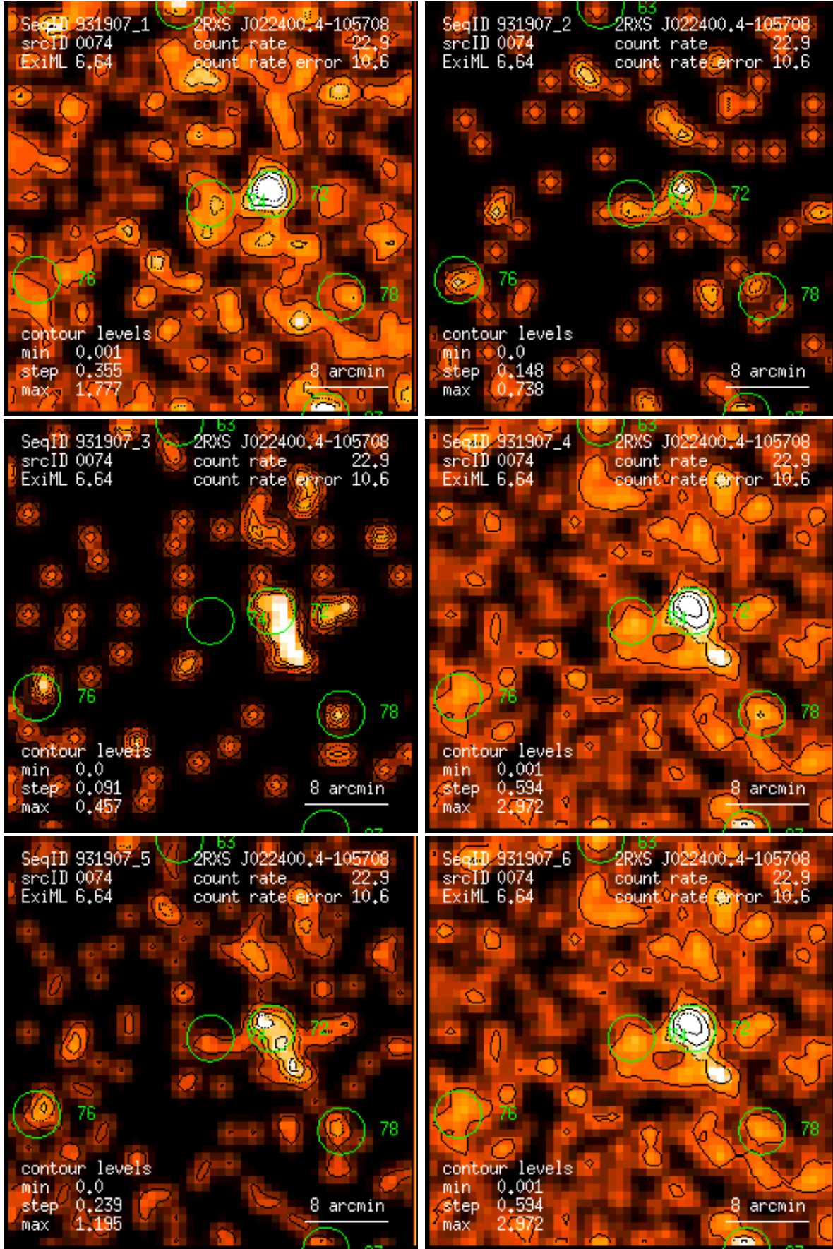
Figure 74: RASS 931907: detection 0074: band rate images, Gaussian filter: (1) PSPC channels 11 – 41, (2) 52 – 90, (3) 91 – 201, (4) 11 – 235, (5) 52 – 201, (6) 11 – 201. Broad band rates in counts/ks. Band rate contour levels in counts/ks/arcmin 2 .
