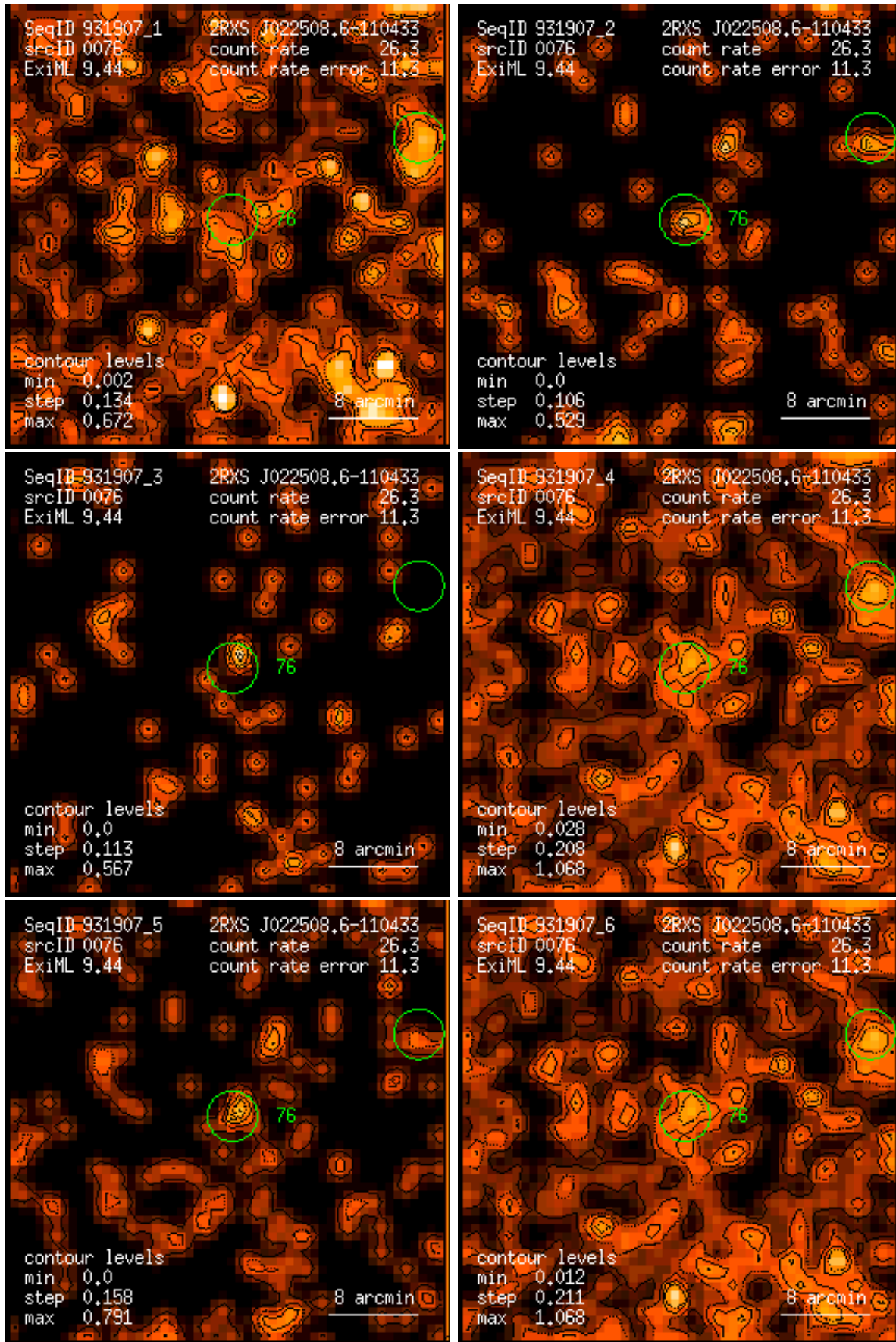
Figure 76: RASS 931907: detection 0076: band rate images, Gaussian filter: (1) PSPC channels 11 – 41, (2) 52 – 90, (3) 91 – 201, (4) 11 – 235, (5) 52 – 201, (6) 11 – 201. Broad band rates in counts/ks. Band rate contour levels in counts/ks/arcmin 2 .
