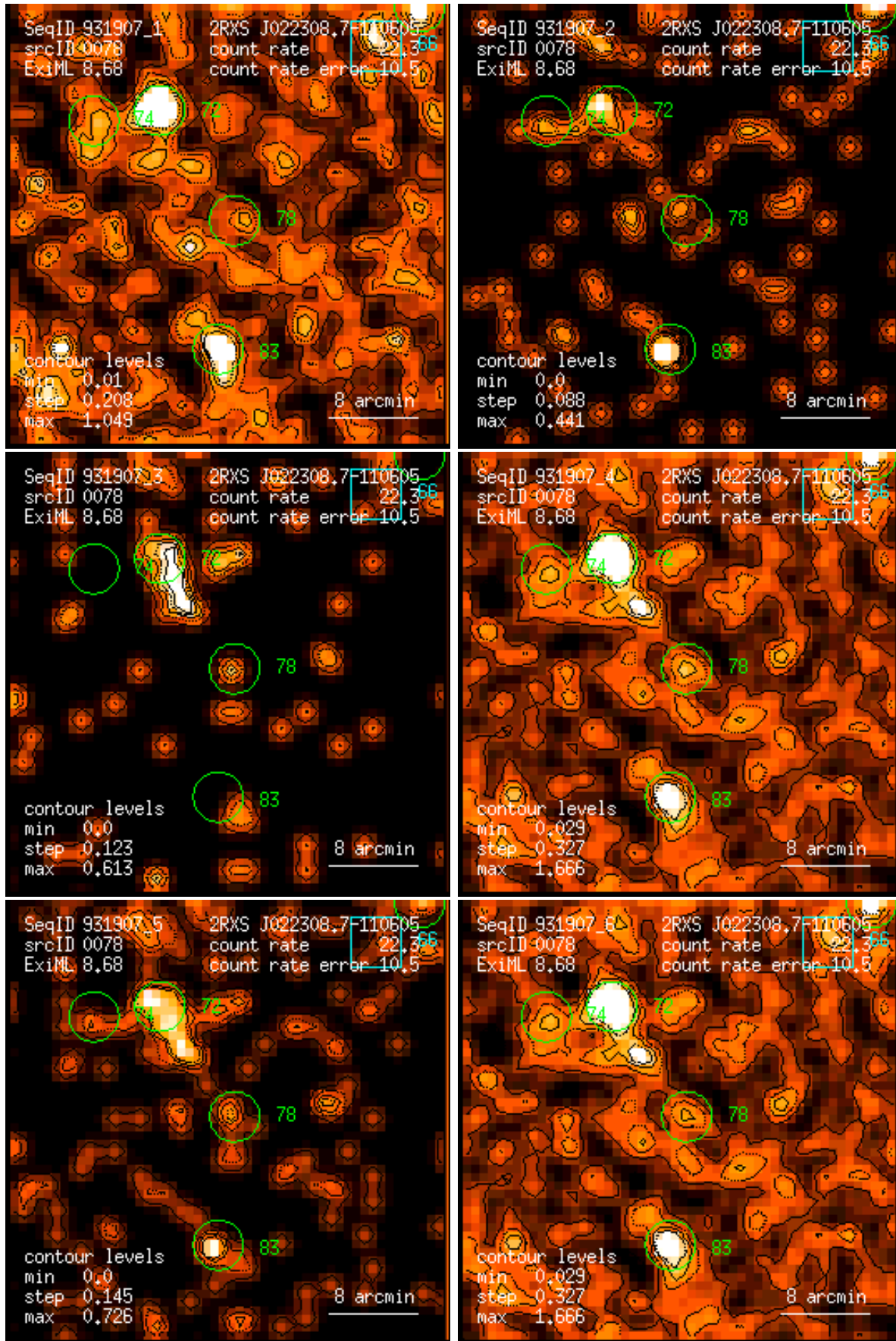
Figure 78: RASS 931907: detection 0078: band rate images, Gaussian filter: (1) PSPC channels 11 – 41, (2) 52 – 90, (3) 91 – 201, (4) 11 – 235, (5) 52 – 201, (6) 11 – 201. Broad band rates in counts/ks. Band rate contour levels in counts/ks/arcmin 2 .
