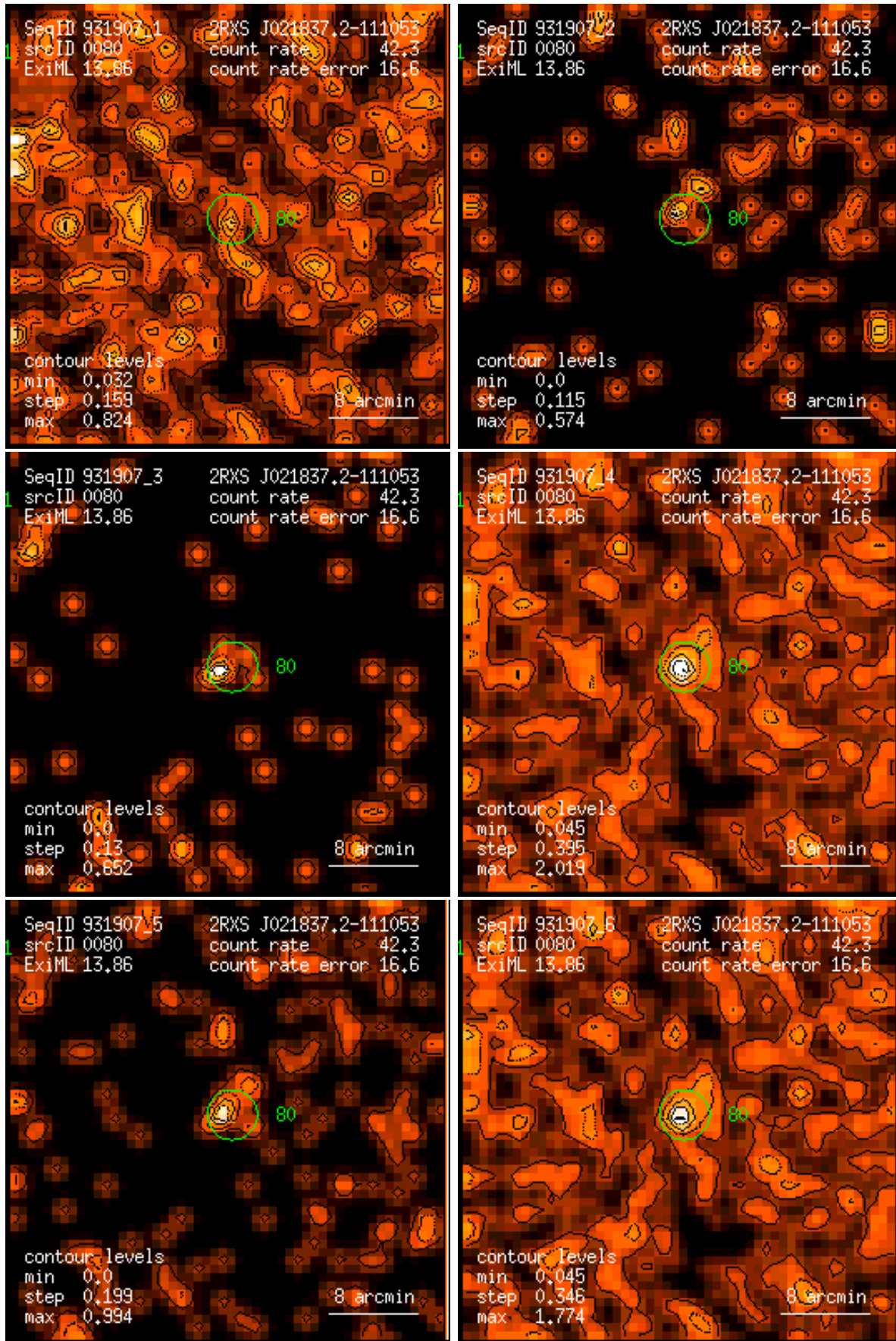
Figure 80: RASS 931907: detection 0080: band rate images, Gaussian filter: (1) PSPC channels 11 – 41, (2) 52 – 90, (3) 91 – 201, (4) 11 – 235, (5) 52 – 201, (6) 11 – 201. Broad band rates in counts/ks. Band rate contour levels in counts/ks/arcmin 2 .
