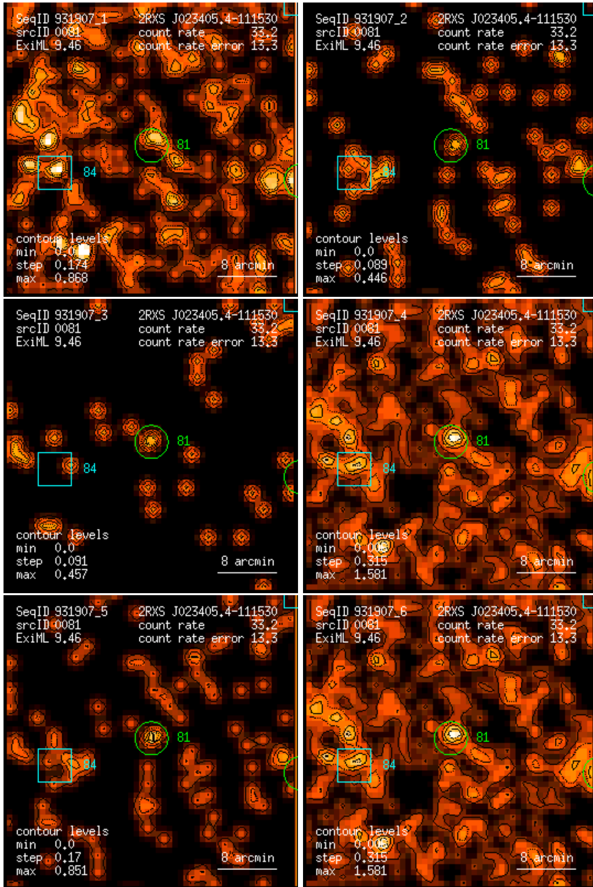
Figure 81: RASS 931907: detection 0081: band rate images, Gaussian filter: (1) PSPC channels 11 – 41, (2) 52 – 90, (3) 91 – 201, (4) 11 – 235, (5) 52 – 201, (6) 11 – 201. Broad band rates in counts/ks. Band rate contour levels in counts/ks/arcmin 2 .
