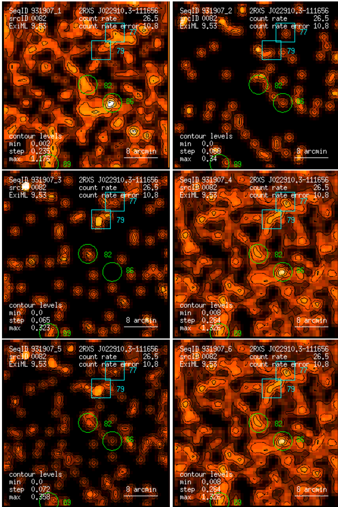
Figure 82: RASS 931907: detection 0082: band rate images, Gaussian filter: (1) PSPC channels 11 – 41, (2) 52 – 90, (3) 91 – 201, (4) 11 – 235, (5) 52 – 201, (6) 11 – 201. Broad band rates in counts/ks. Band rate contour levels in counts/ks/arcmin 2 .
