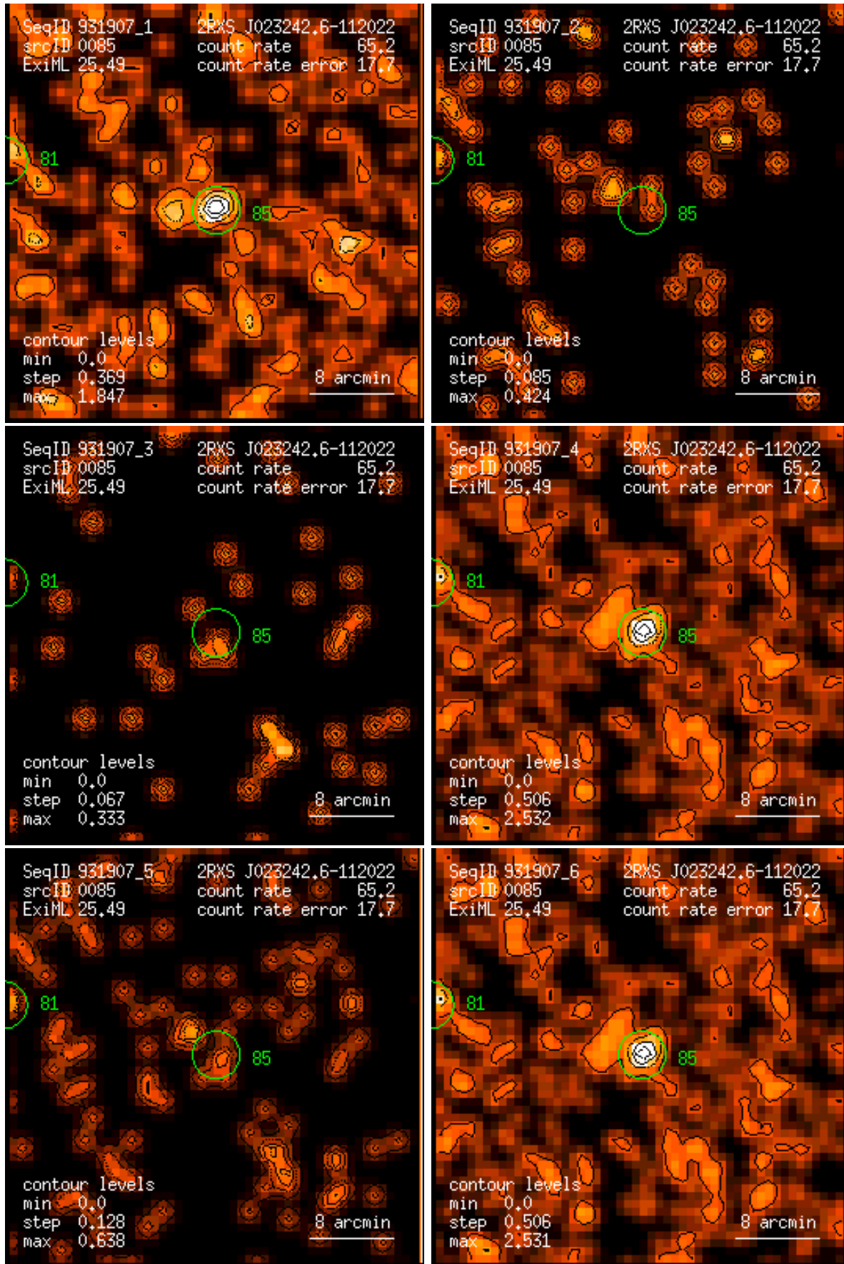
Figure 85: RASS 931907: detection 0085: band rate images, Gaussian filter: (1) PSPC channels 11 – 41, (2) 52 – 90, (3) 91 – 201, (4) 11 – 235, (5) 52 – 201, (6) 11 – 201. Broad band rates in counts/ks. Band rate contour levels in counts/ks/arcmin 2 .
