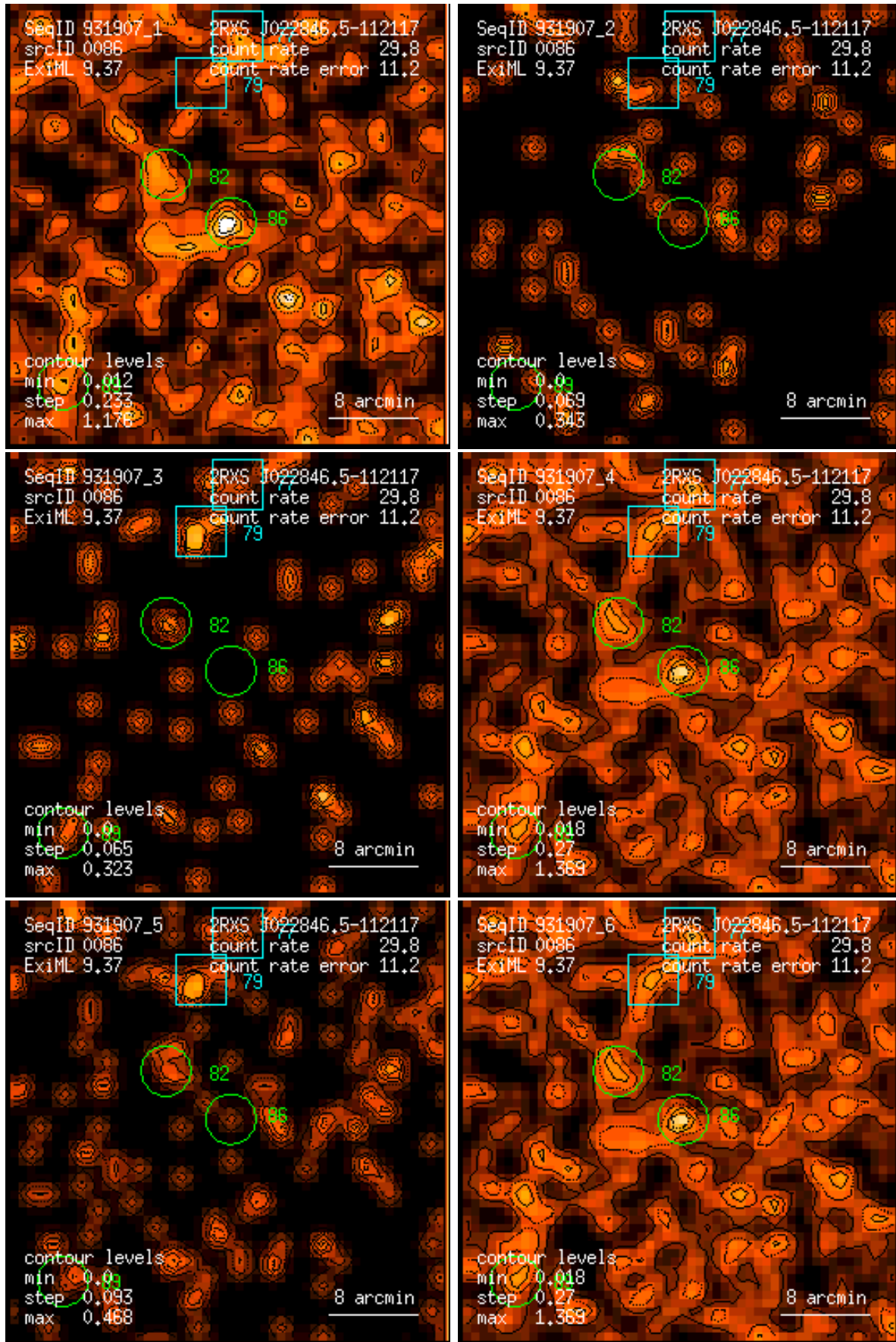
Figure 86: RASS 931907: detection 0086: band rate images, Gaussian filter: (1) PSPC channels 11 – 41, (2) 52 – 90, (3) 91 – 201, (4) 11 – 235, (5) 52 – 201, (6) 11 – 201. Broad band rates in counts/ks. Band rate contour levels in counts/ks/arcmin 2 .
